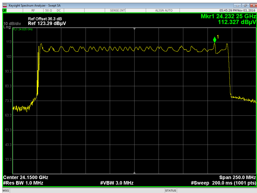
Plot No. 1: Peak measurement, Mode 1
