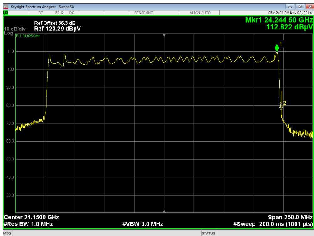
Plot No. 2: Peak measurement, Mode 2
