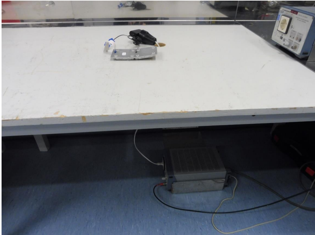
Photo 1: Conducted emissions
