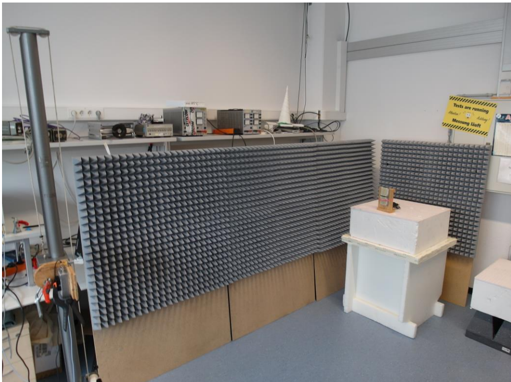
Photo 8: RSE set-up 18 GHz to 110 GHz
