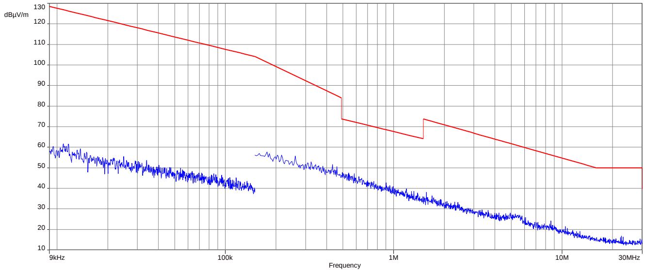
Plot 7: TX Magnetic, 9 kHz – 30 MHz, SMR 333, horizontal / vertical polarization
