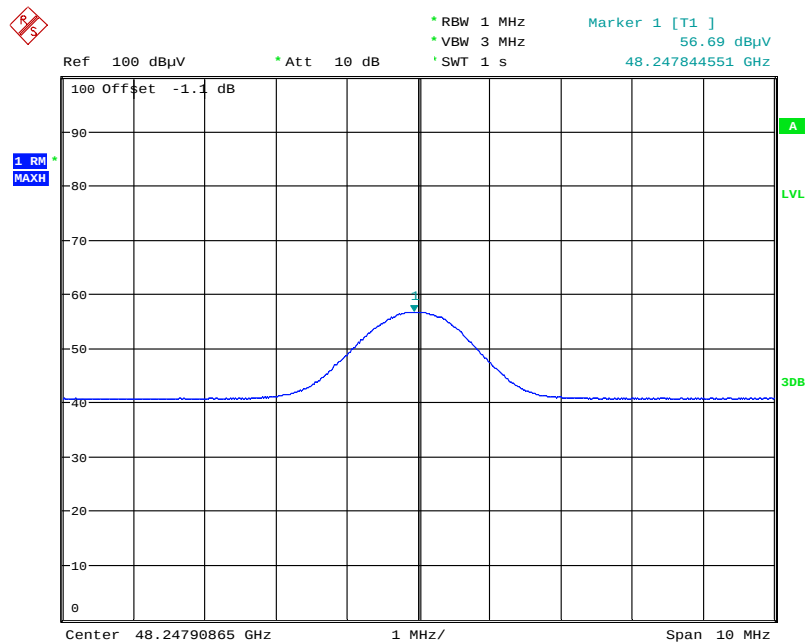
Plot 14: 1 st harmonic, SMR 333, horizontal / vertical polarization
