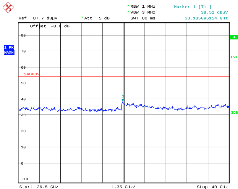
Plot 12: 26.5 GHz to 40 GHz, horizontal / vertical polarization
