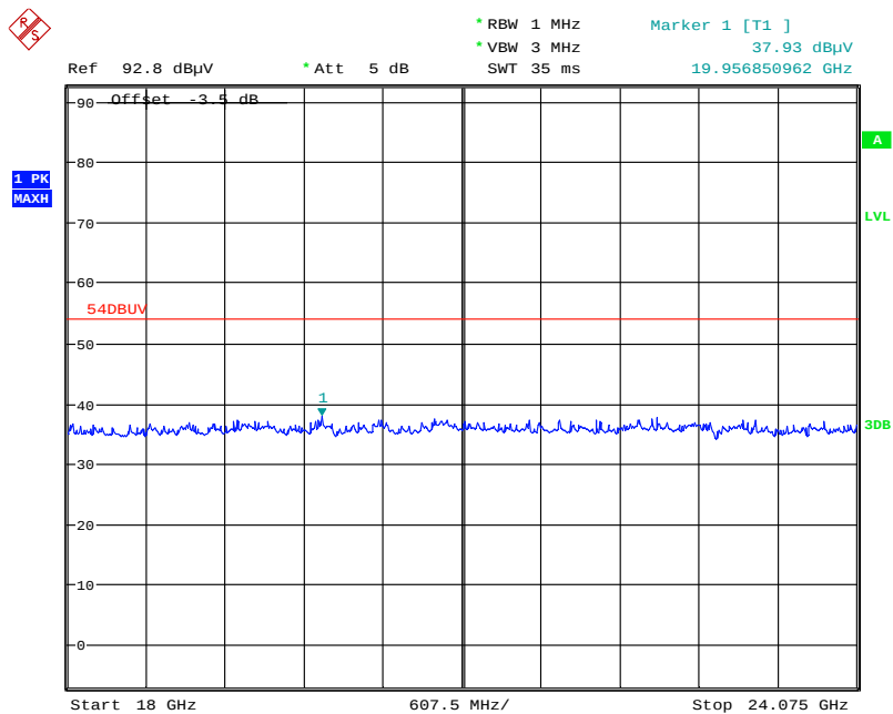
Plot 10: 18 GHz to 24.075 GHz, SMR 333, horizontal / vertical polarization
