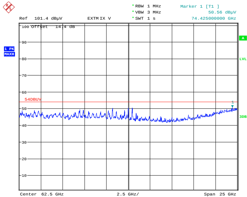
Plot 15: 50 GHz to 75 GHz, horizontal / vertical polarization
