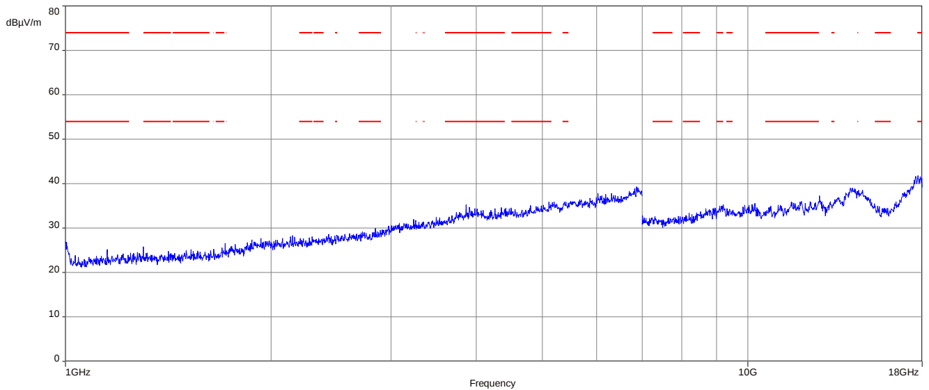
Plot 9: 1 GHz to 18 GHz, SMR 333, horizontal / vertical polarization
