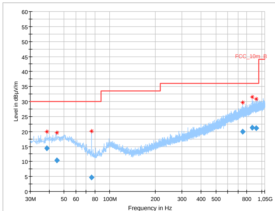
Plot 8: 30 MHz to 1 GHz, SMR 333, horizontal / vertical polarization
