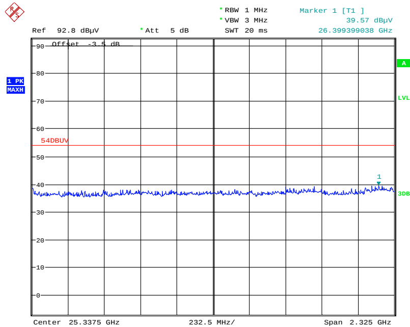
Plot 11: 24.175 GHz to 26.5 GHz, SMR 333, horizontal / vertical polarization
