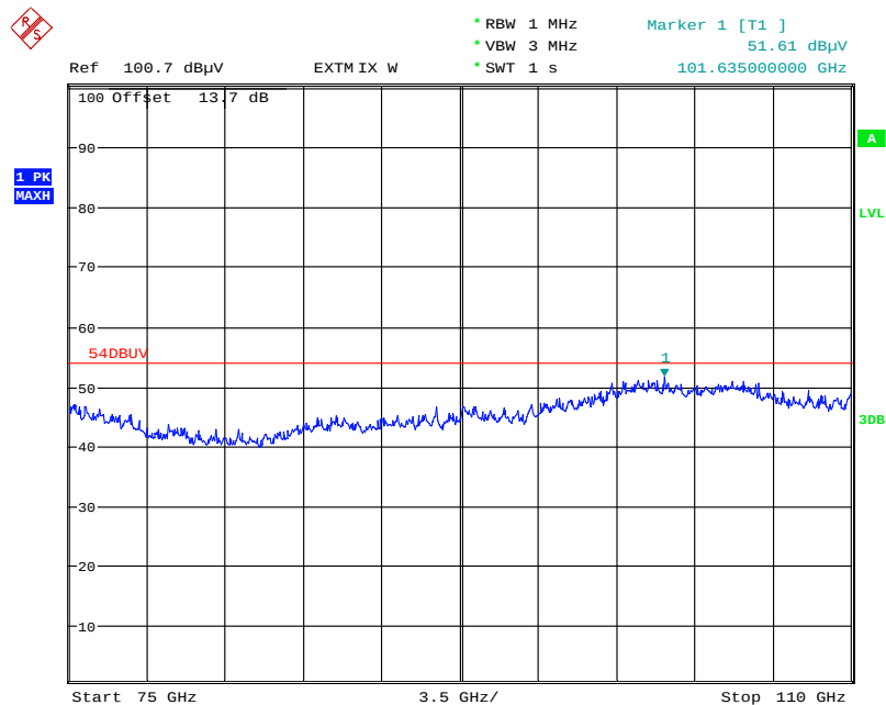
Plot 16: 75 GHz to 110 GHz, horizontal / vertical polarization
