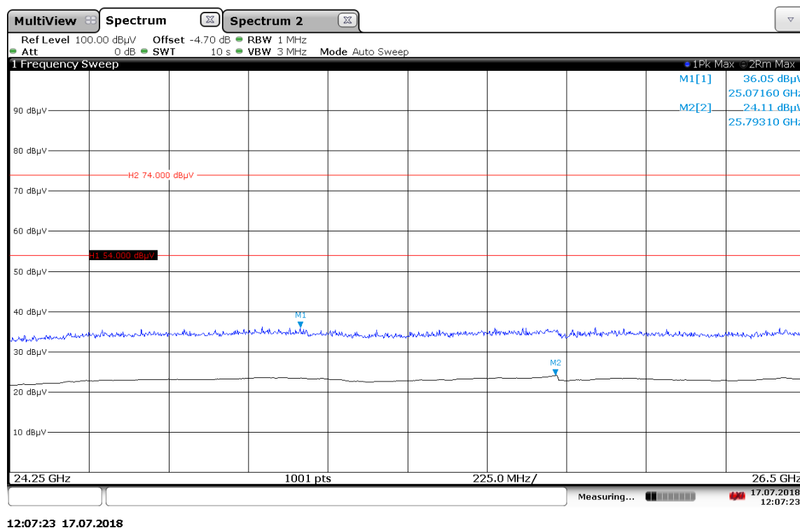
Plot No. 8: 24.25 GHz to 26.5 GHz, horizontal / vertical polarization
