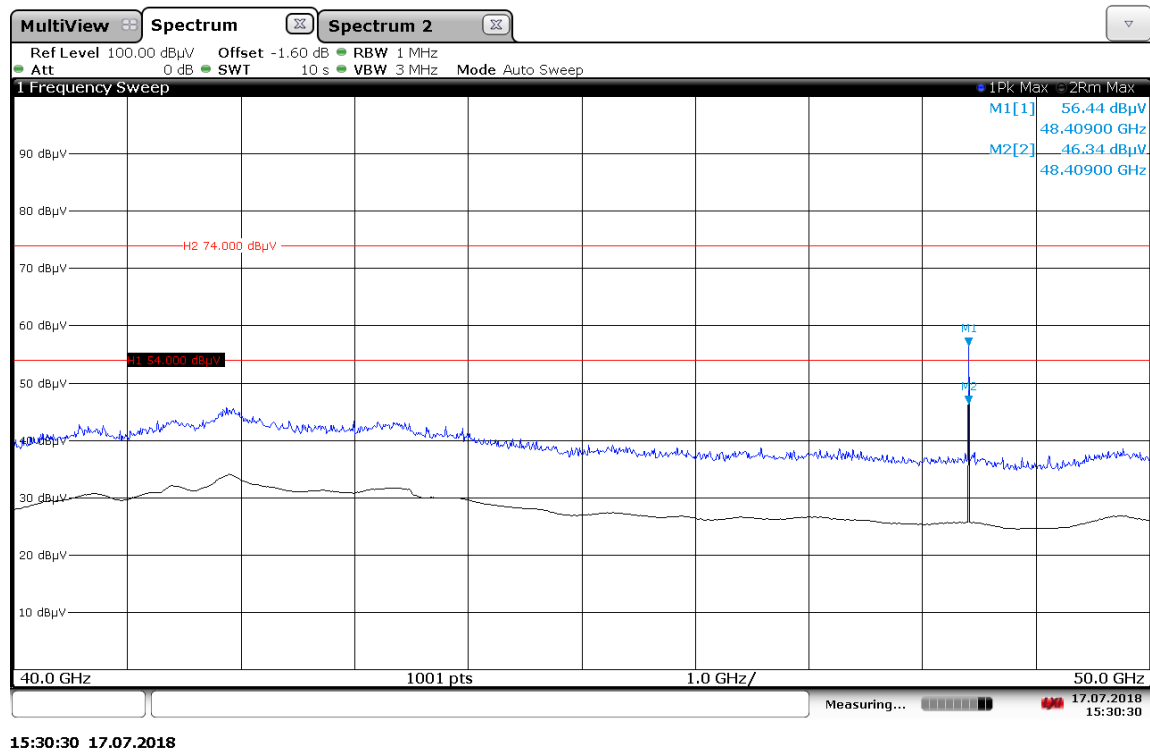
Plot No. 10: 40 GHz to 50 GHz, horizontal / vertical polarization
