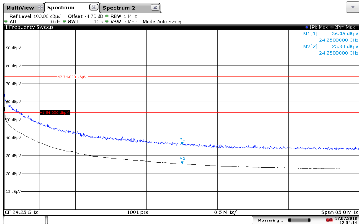
Plot No. 7: Band-Edge-Compliance, upper band-edge
