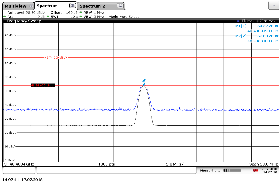
Plot No. 11: Second harmonic
