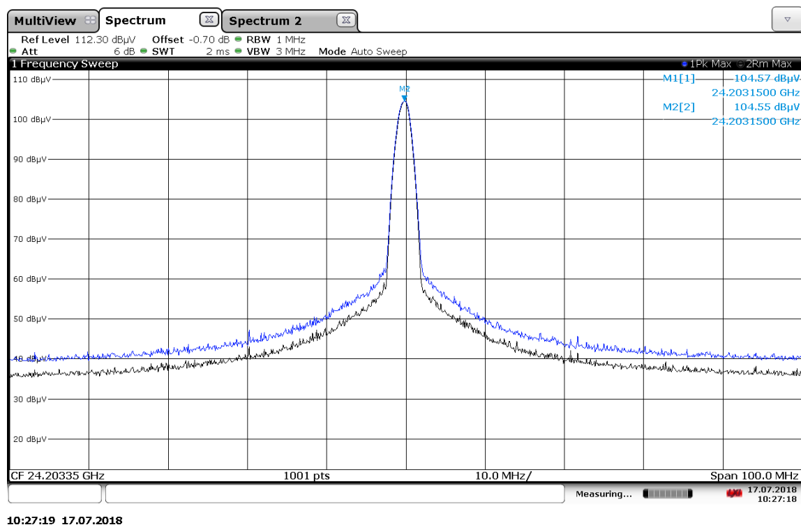
Plot No. 1: Peak measurement, normal operation mode
