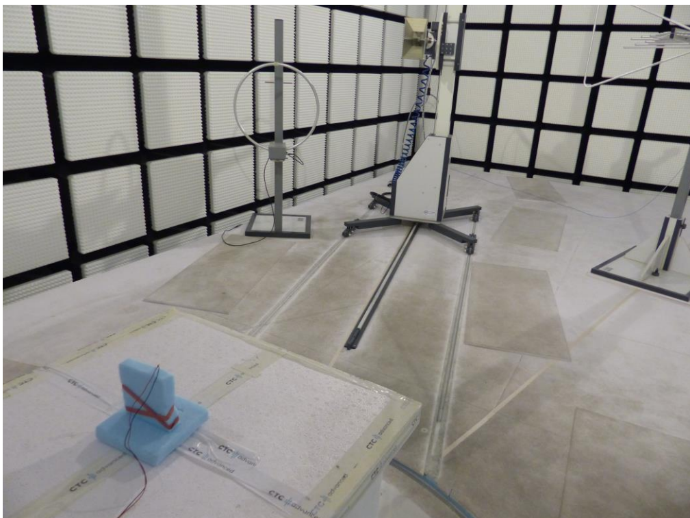
Photo 6: Set-up 9 kHz to 30 MHz
