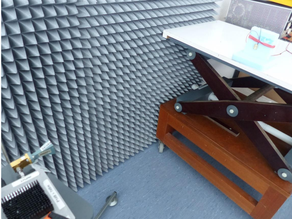
Photo 7: Set-up 18 GHz to 110 GHz
