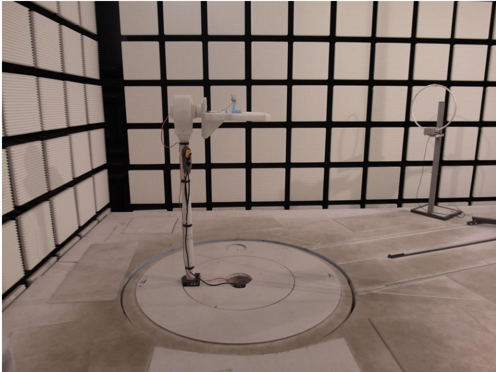
Photo 1: RSE set-up 1 GHz to 18 GHz
