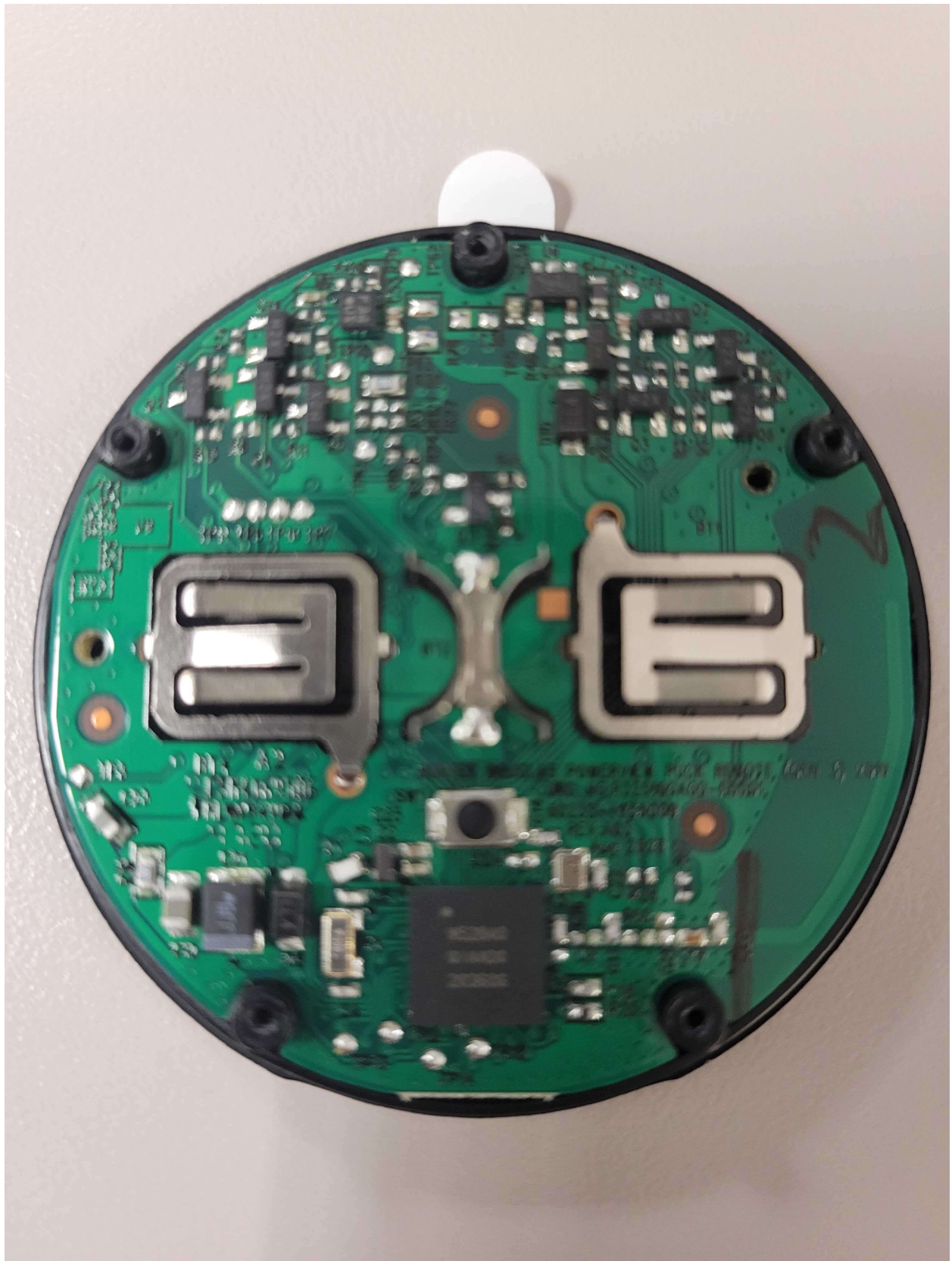
Photo – Internal Front
