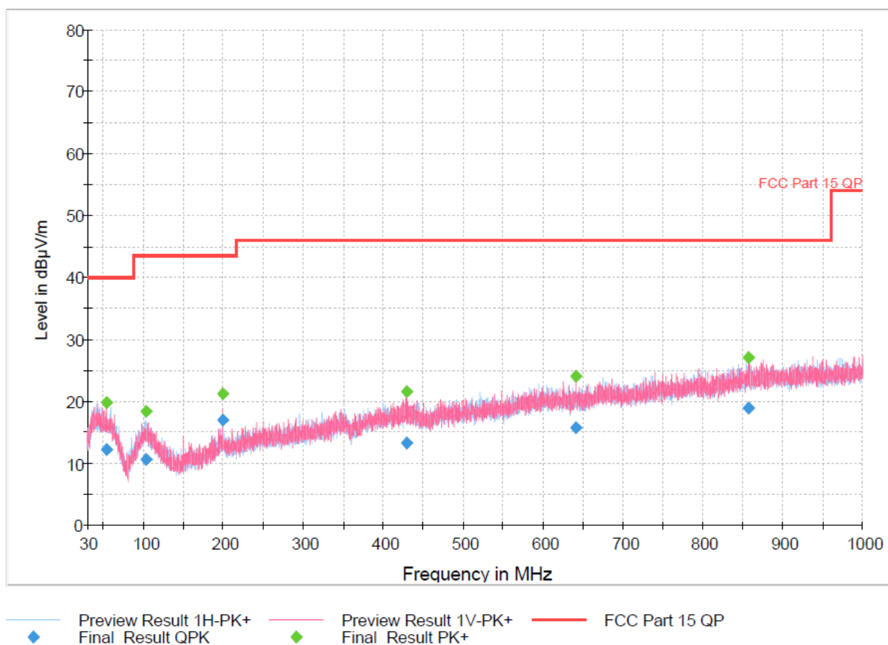
Figure 44: Radiated Spurious Emissions 30MHz – 1GHz, 2440MHz, 2Mbps
