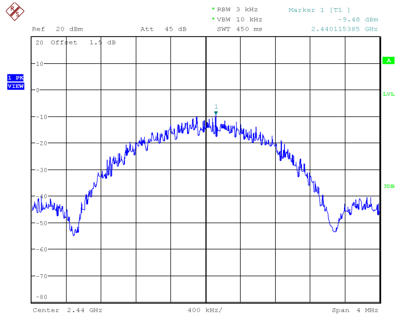
Figure 25: 2440 MHz, 2Mbps, PSD
