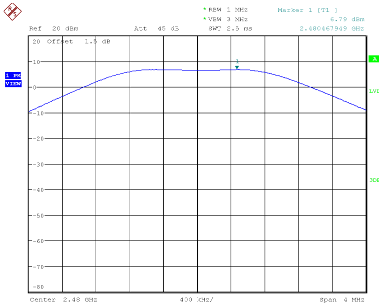
Figure 8: Maximum Conducted Power, 2480MHz, 2Mbps
