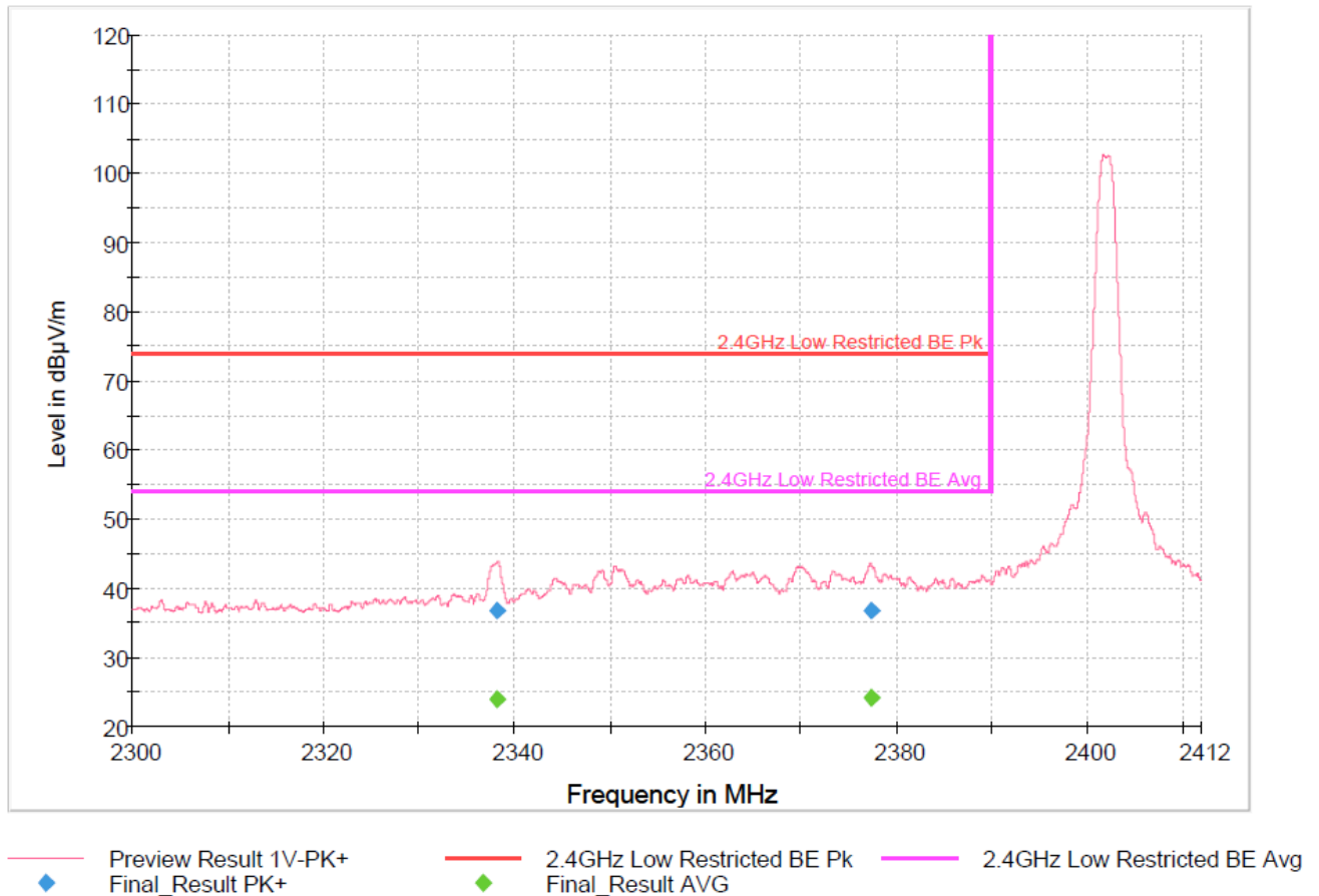
Figure 39: Restricted Band Edge, Low, 2402MHz, 1 Mbps
