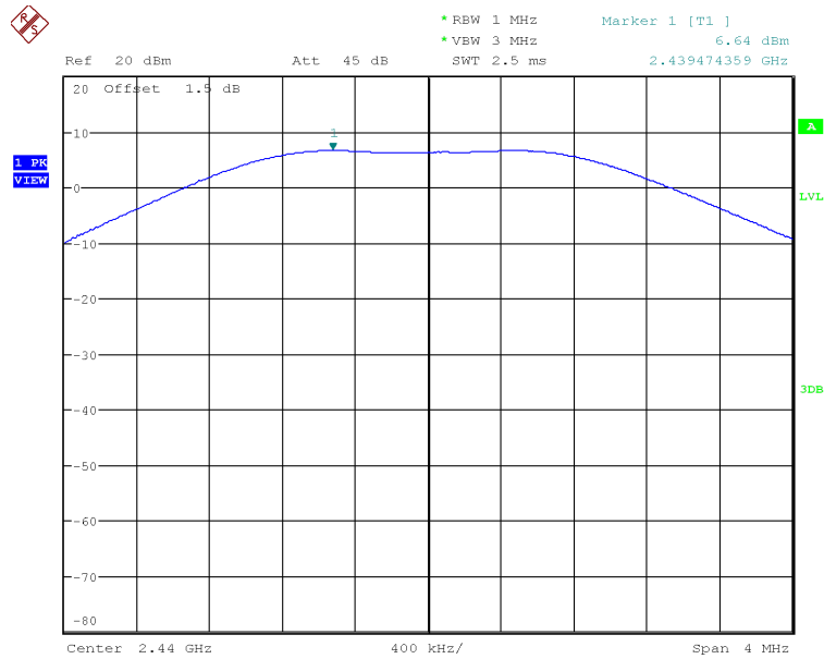
Figure 7: Maximum Conducted Power, 2440MHz, 2Mbps
