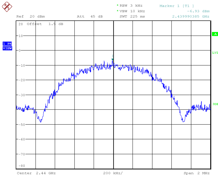
Figure 22: 2440 MHz, 1Mbps, PSD
