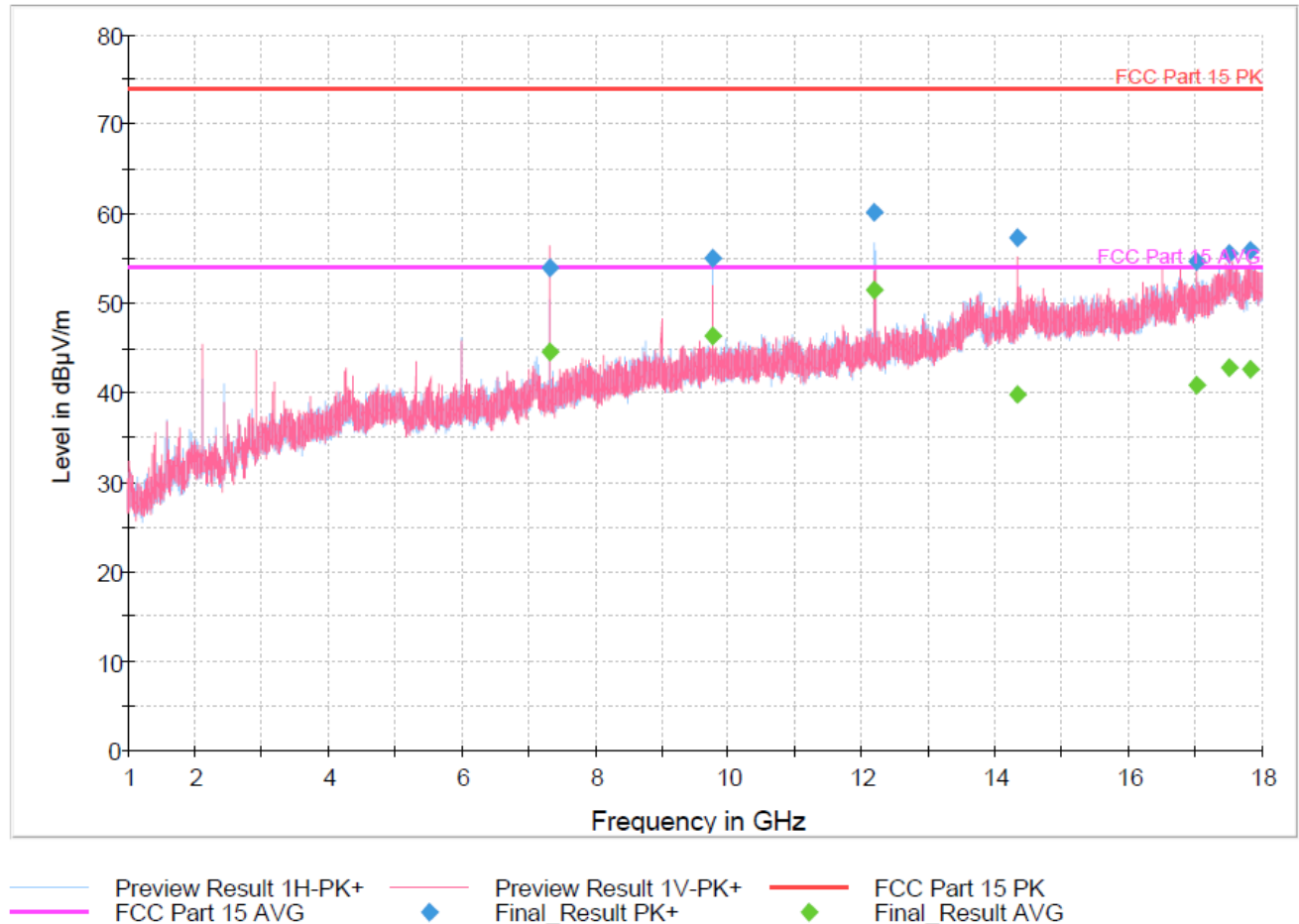
Figure 49: Radiated Spurious Emissions 1GHz - 18GHz, 2440MHz, 2Mbps
