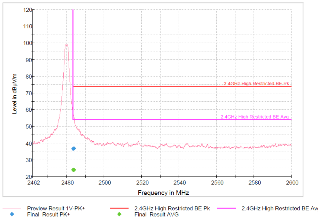
Figure 42: Restricted Band Edge, High, 2480MHz, 2 Mbps
