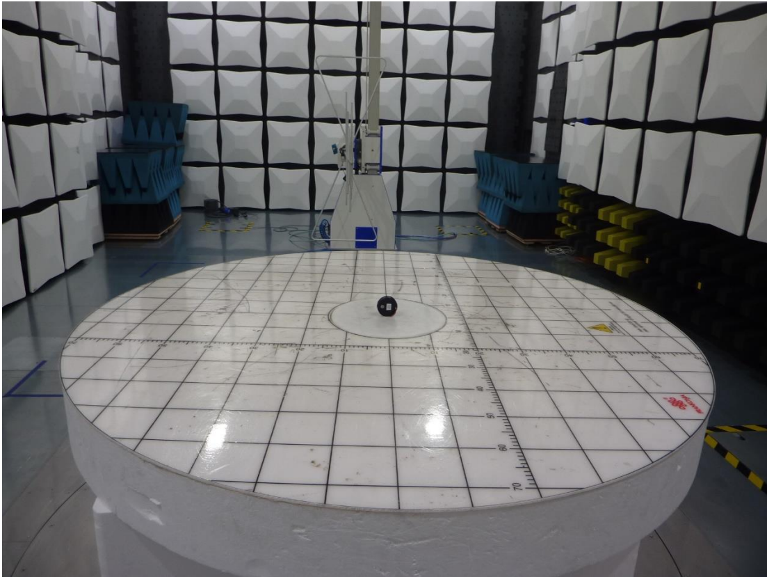
Figure 2: Test Setup for 30 MHz to 1 GHz (View 2)
