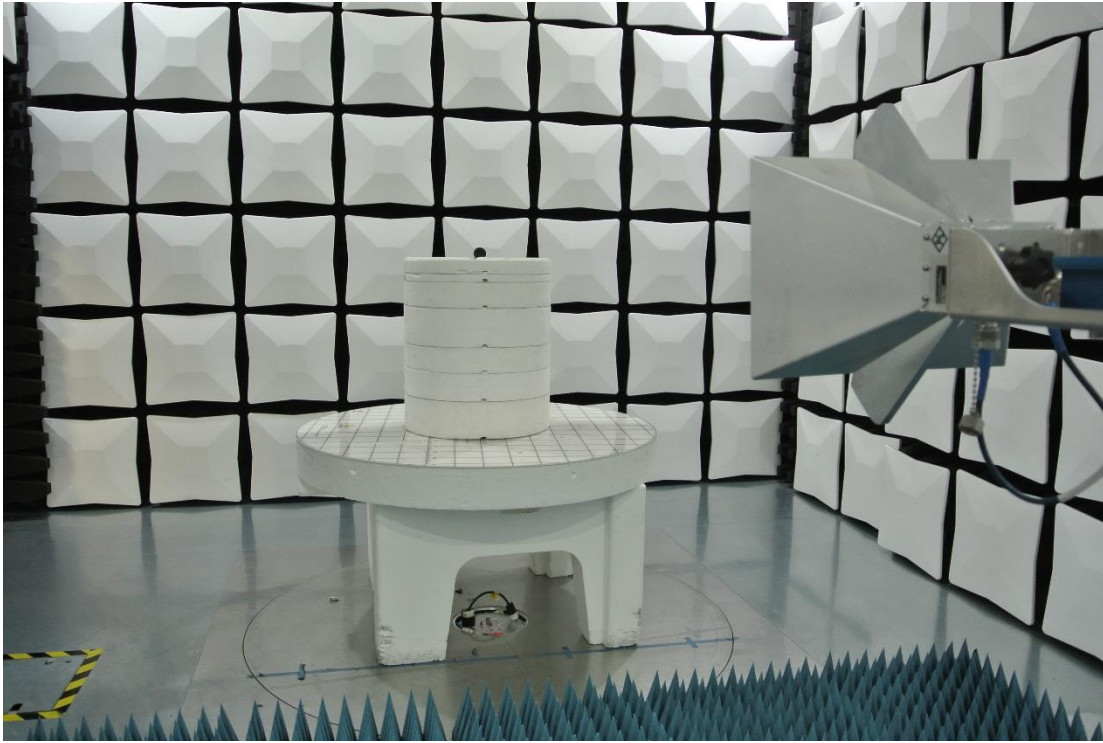
Figure 3: Test Setup for 1 GHz to 18 GHz (View 1)
