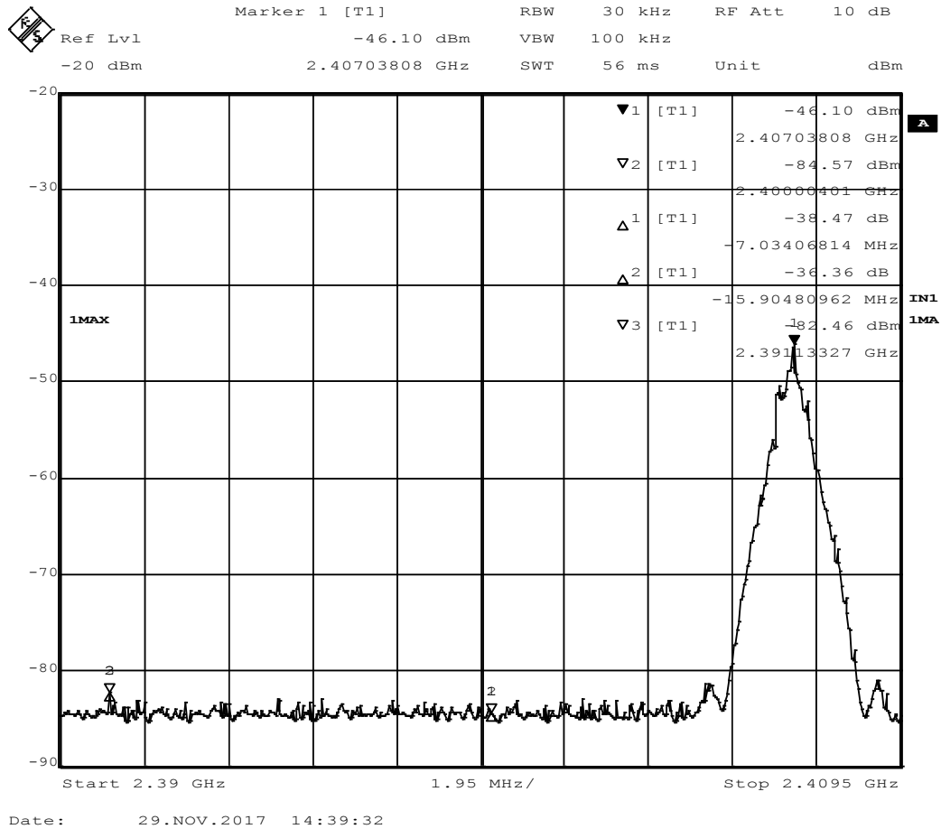
Figure 18 - Band-edge Measurement, Low Channel, Fundamental
