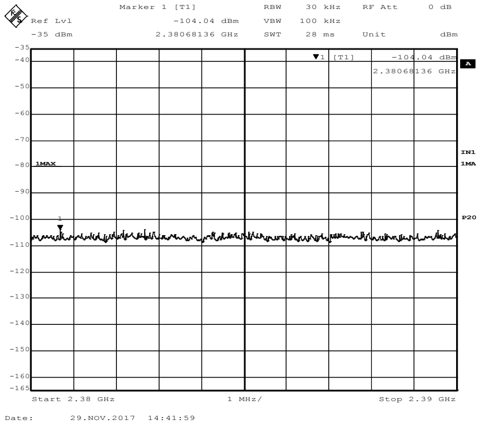
Figure 17 - Band-edge Measurement, Low Channel, Restricted Frequency
