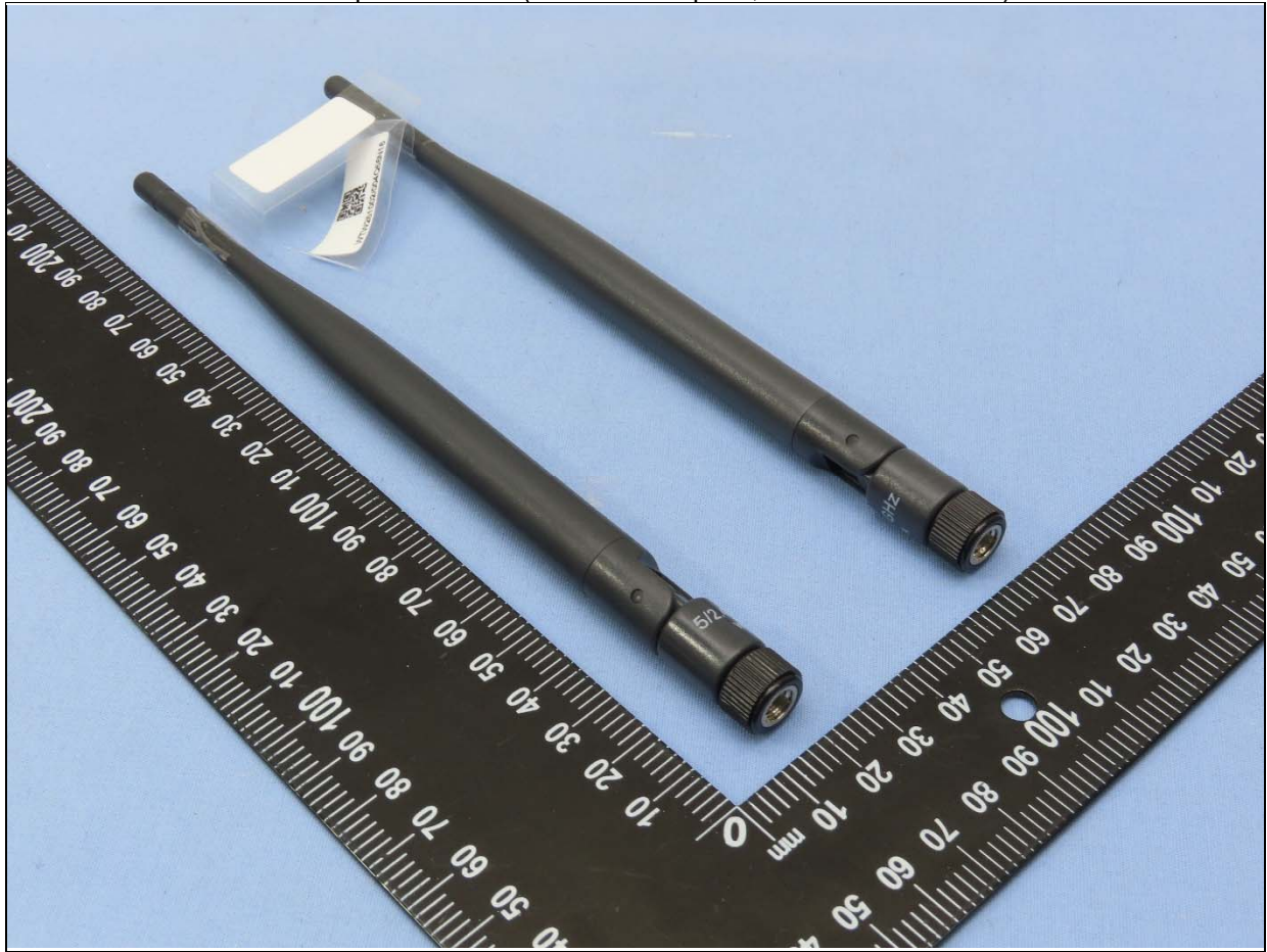
WiFi: Dipole Antenna (Brand: cradlepoint, Model: 170836-000)
