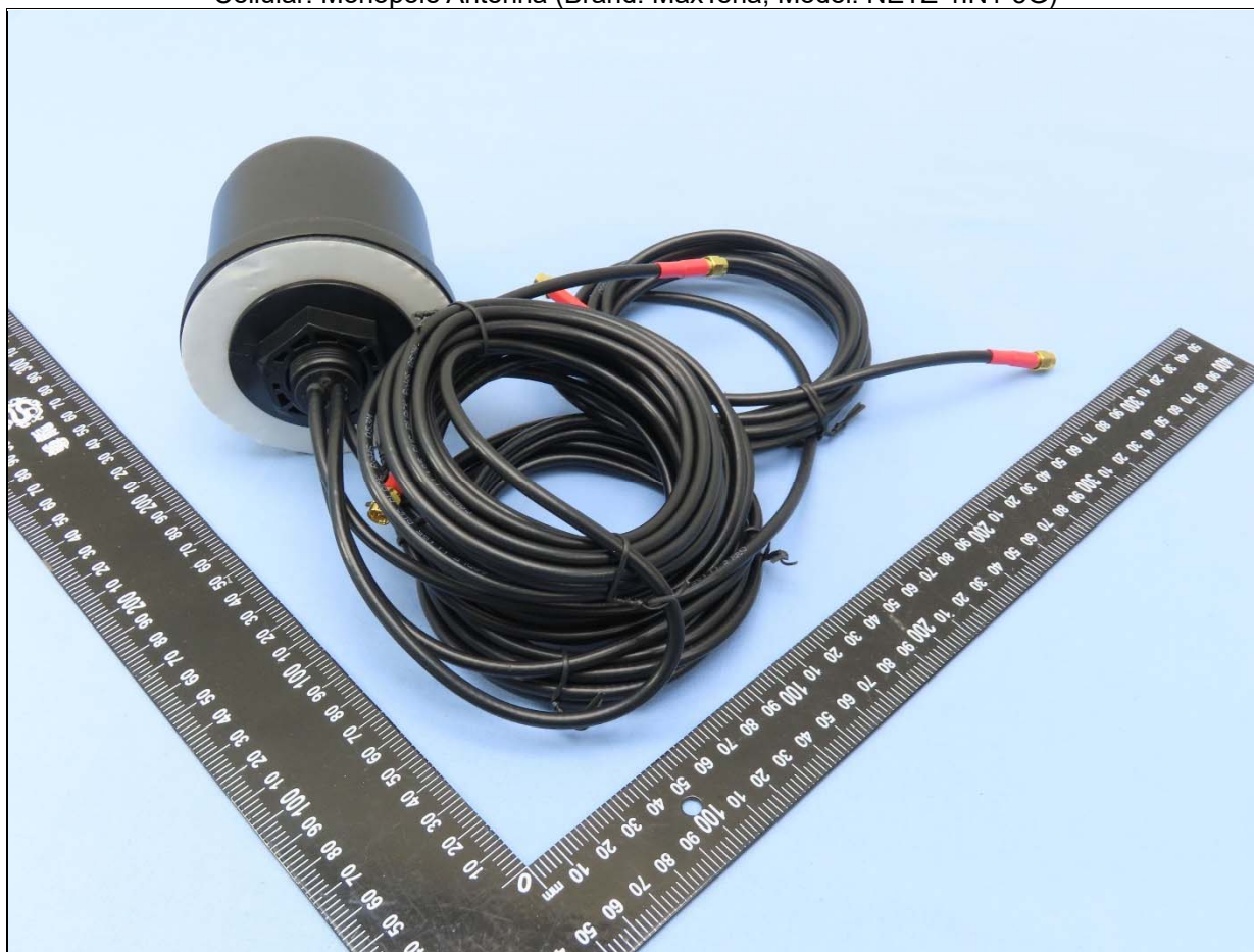
Cellular: Monopole Antenna (Brand: MaxTena, Model: NETZ 4IN1-5G)
