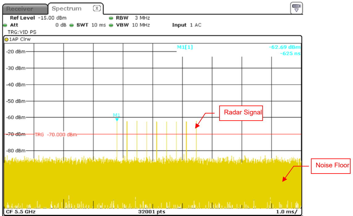
Radar Signal 6
