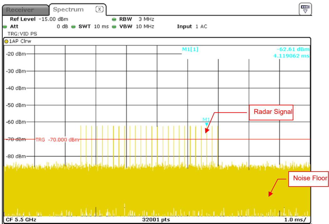
Radar Signal 2
