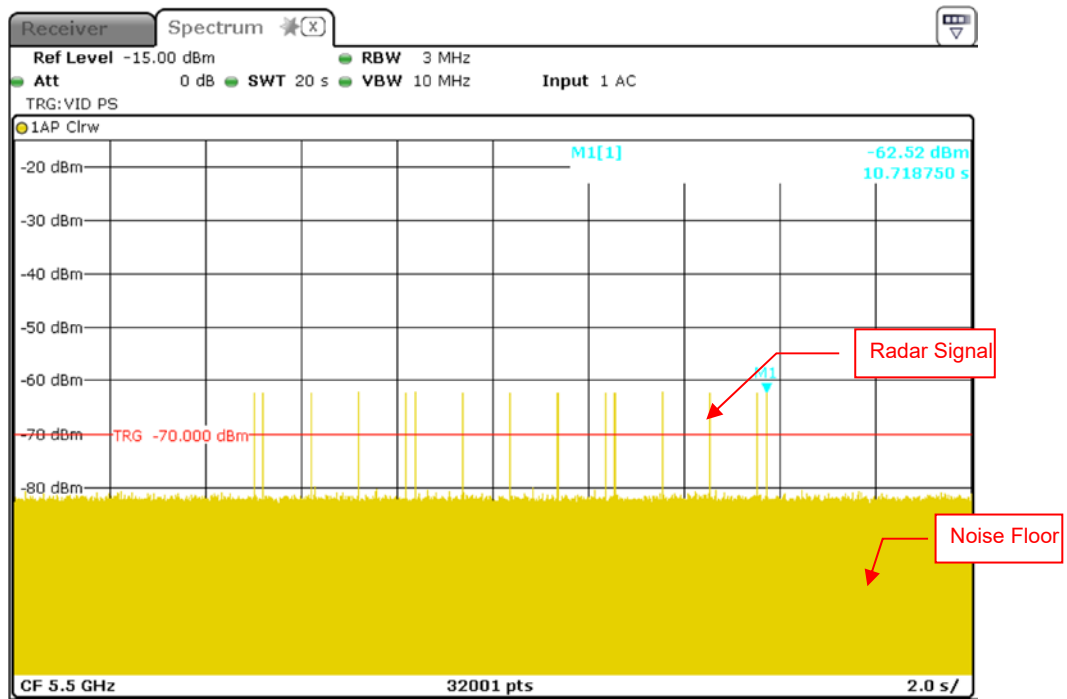
Radar Signal 5
