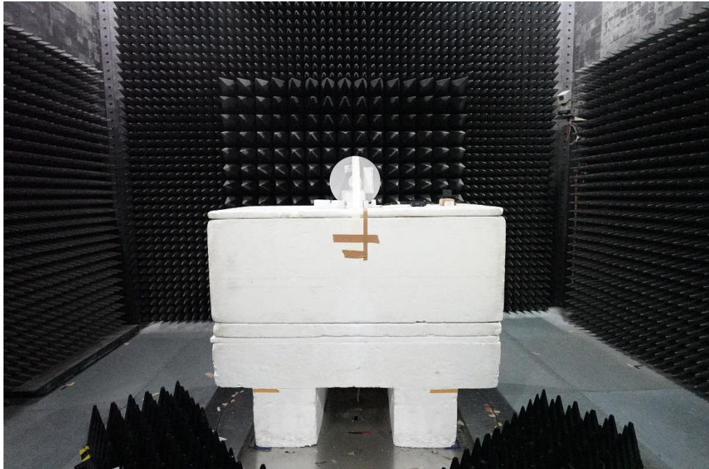
Monopole Antenna
