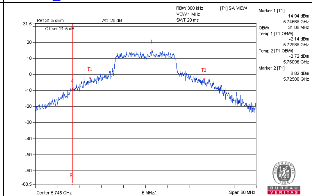
802.11ac(VHT20)_Chain1 / CH149
