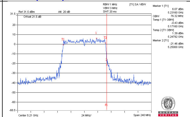
802.11ac(VHT80)_Chain1 / CH42
