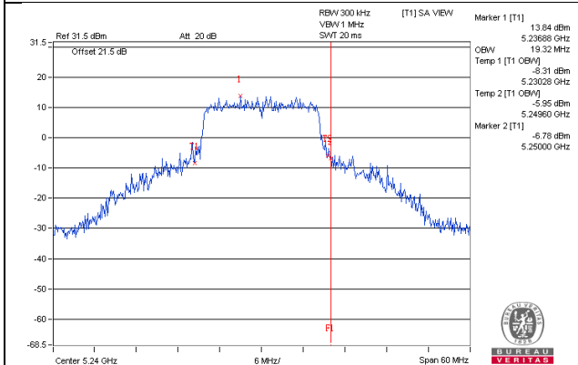
802.11ac(VHT20)_Chain0 / CH48
