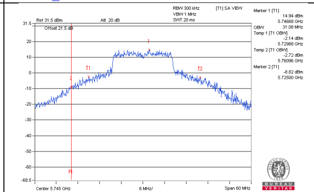
802.11ac(VHT20)_Chain1 / CH149
