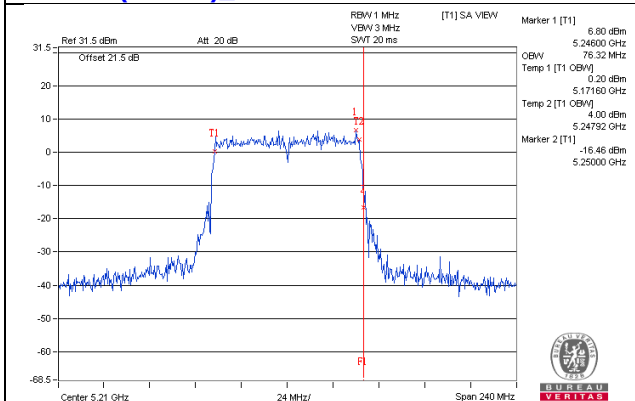
802.11ac(VHT80)_Chain0 / CH42
