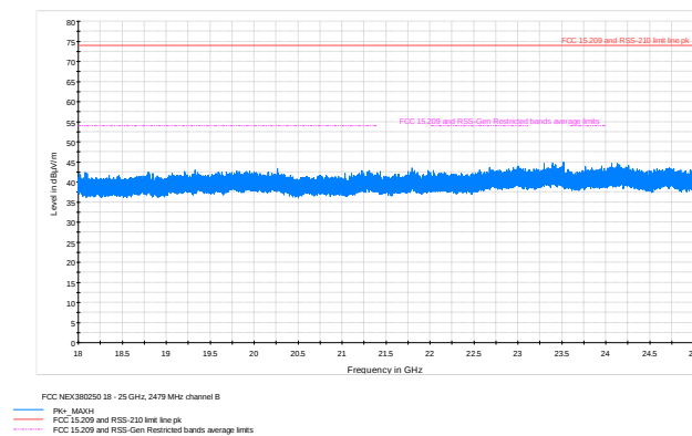
Figure 8.6-34: Radiated spurious emissions 18 - 25 GHz, 2479 MHz, Channel B
