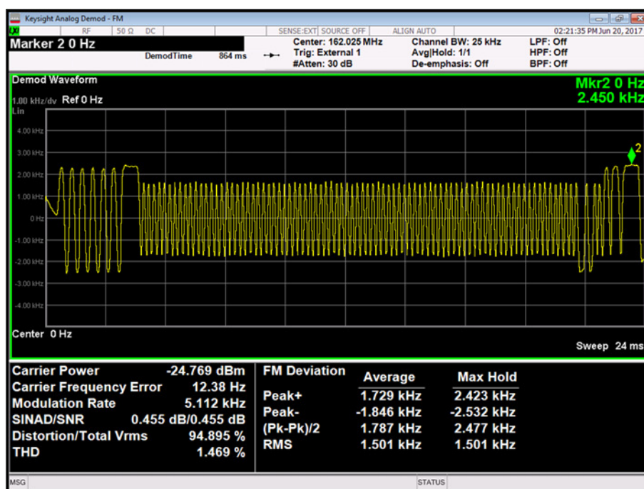
Figure 22 - 162.025 MHz - 01010101
