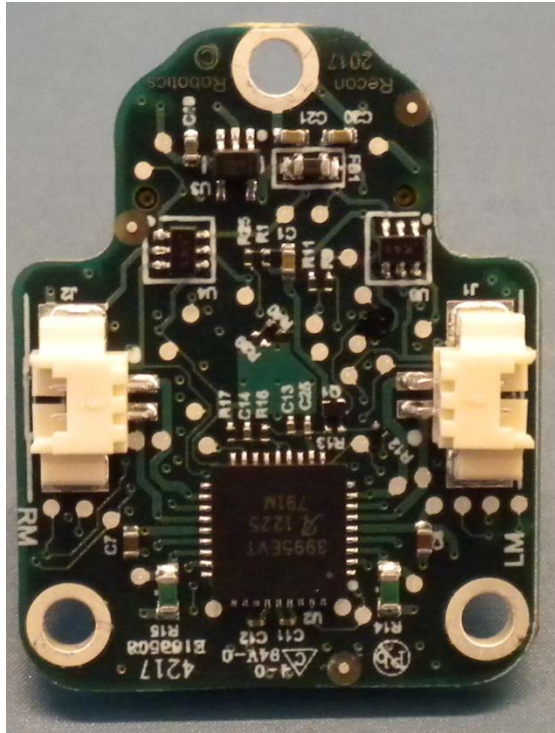
Figure 5: Interface Board, Back
