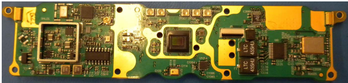
Figure 2: Main Board, Front (shield cover not installed)
