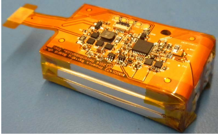
Figure 11: Battery Board installed in Battery Assembly (heat shrink removed)
