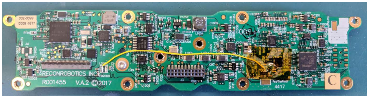
Figure 1: Main Board, Back
