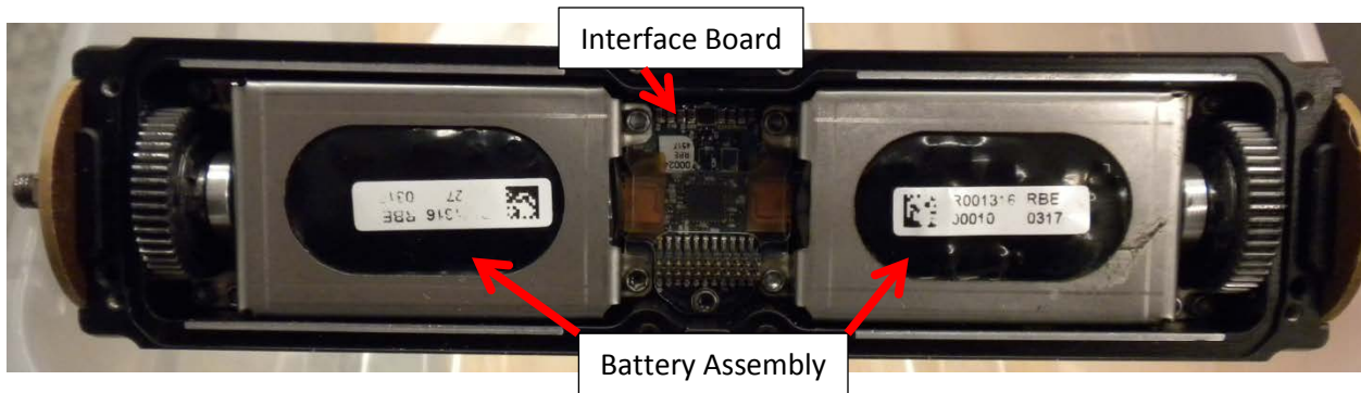
Figure 13: Interface Board and Batteries (2x) Installed
