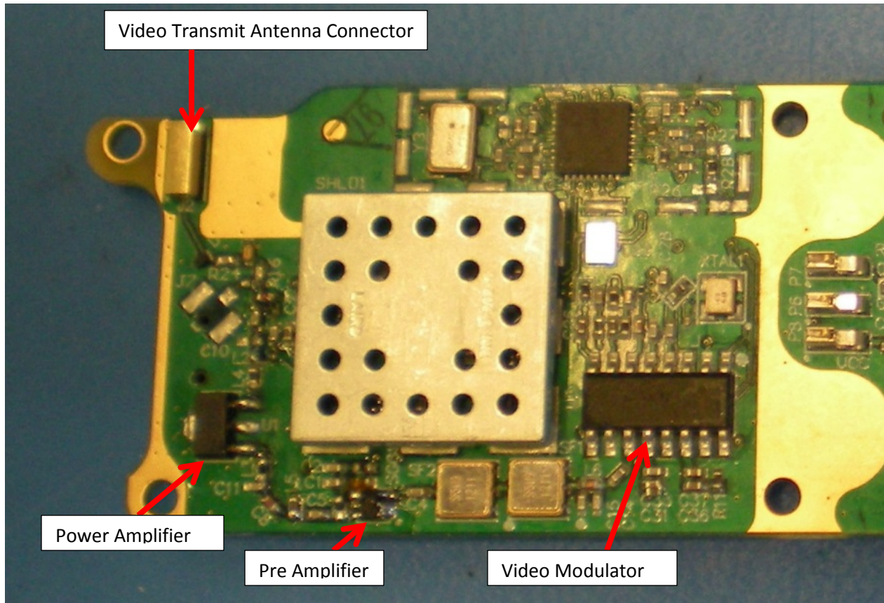
Figure 4: Main Board, Front (annotated functionality)
