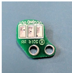
Figure 5: Hall Sensor Board, Back
