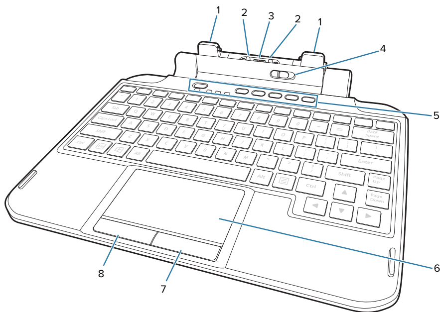
Figure 8 ET80/ET85 Keyboard Features
