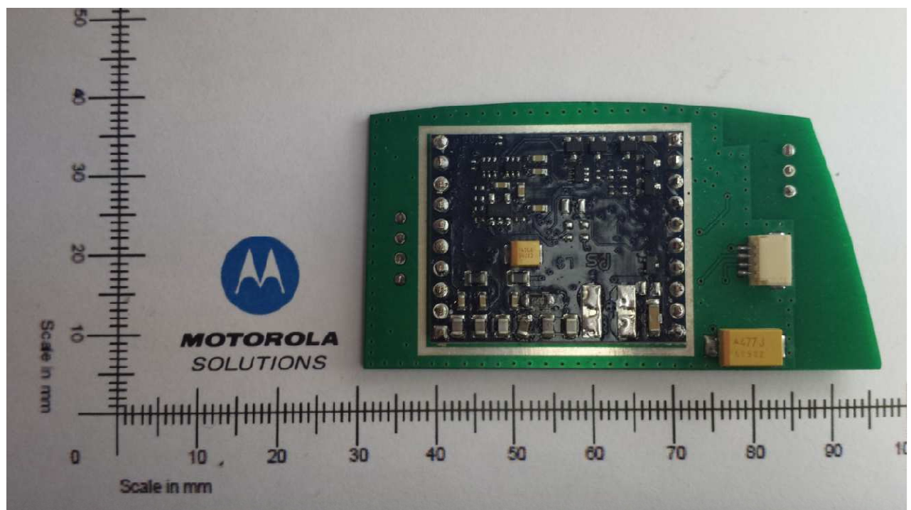
TOP VIEW WITH LF OEM
