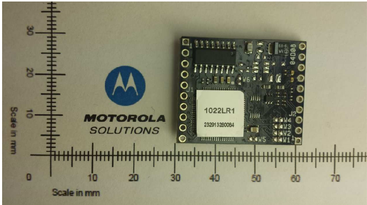
TOP VIEW
