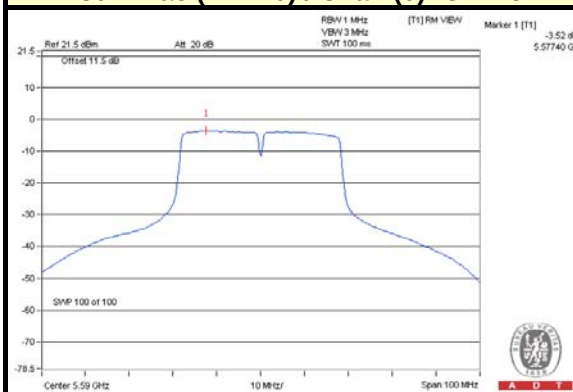
802.11ac (VHT40) / Chain(0): CH118
