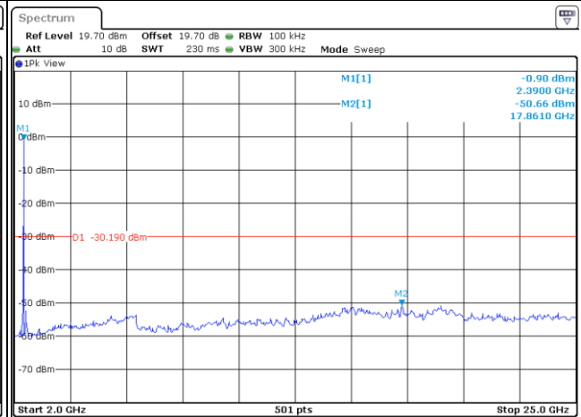
Conducted Spurious Emission Plot on Bluetooth LE 2Mbps GFSK Channel 00
