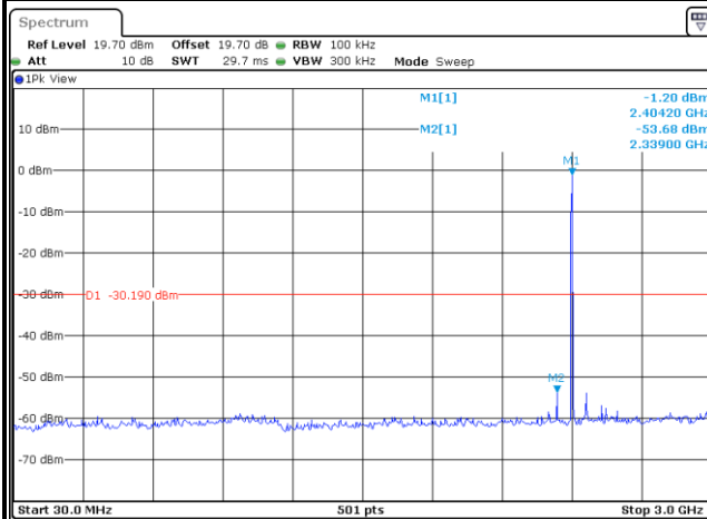
Conducted Spurious Emission Plot on Bluetooth LE 2Mbps GFSK Channel 00
