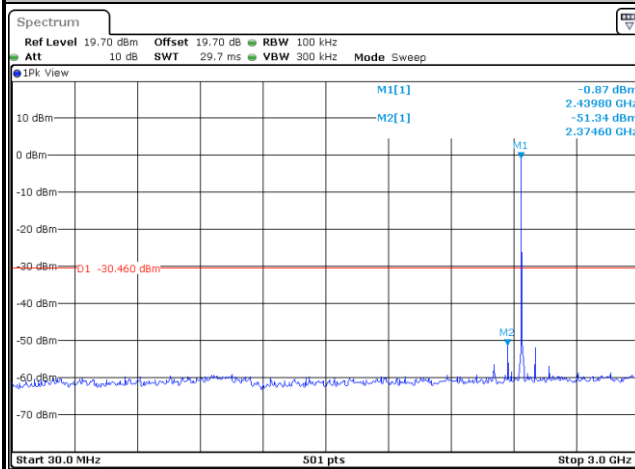
Conducted Spurious Emission Plot on Bluetooth LE 2Mbps GFSK Channel 19
