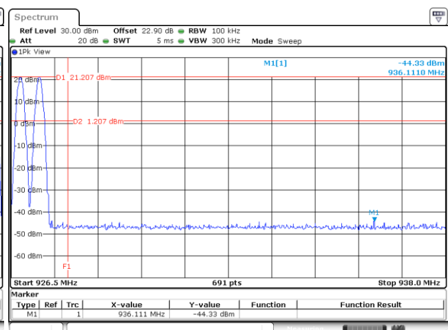
Hopping Mode High Band Edge Plot on 927.25 MHz
