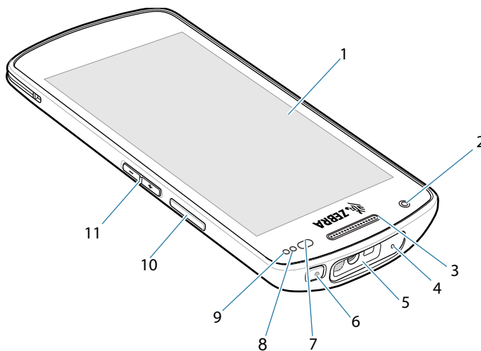
Figure 1 Front View
