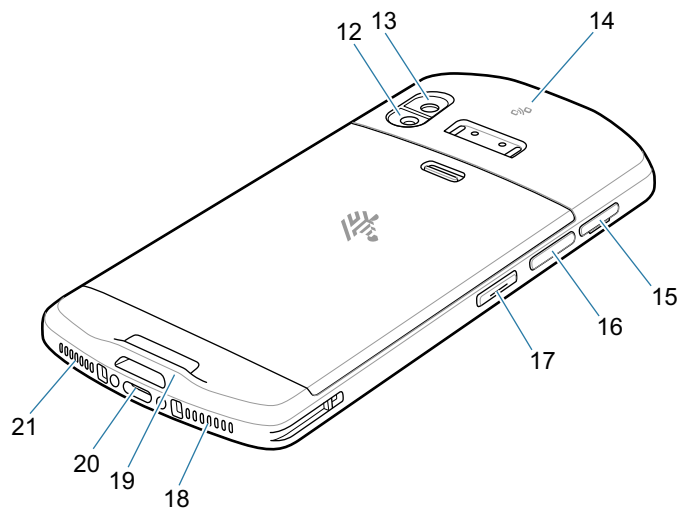
Figure 2 Rear View
