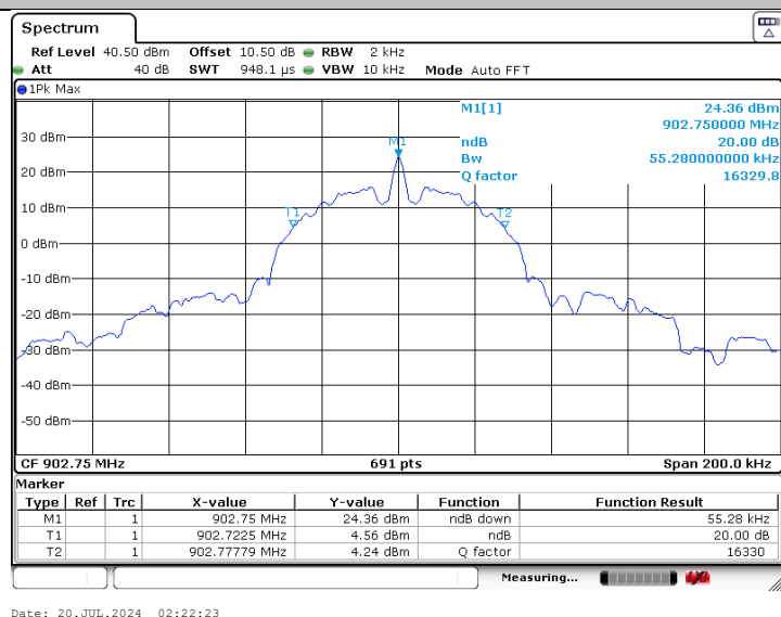
20 dB Bandwidth Plot on 902.75 MHz
