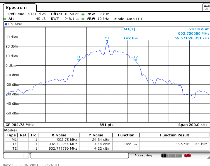
99% Occupied Bandwidth Plot on 902.75 MHz
