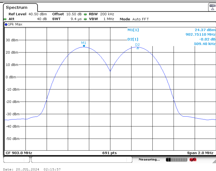
Channel Separation Plot on 902.75 MHz
