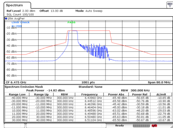
Plot on Channel 6475MHz 52RU37
