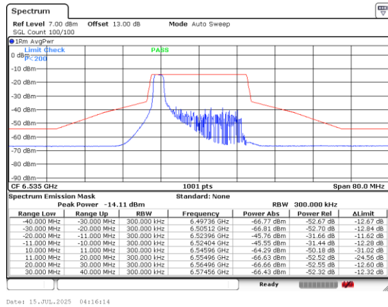
Plot on Channel 6535MHz 106RU53
