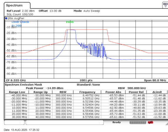
Plot on Channel 6535MHz 52RU37
