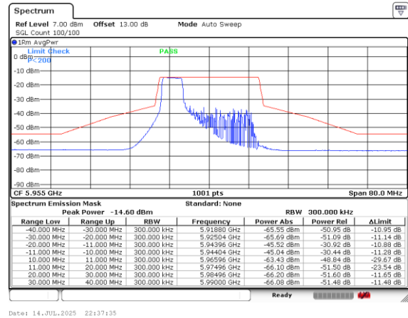
Plot on Channel 5955MHz Small RUs-52+2638
