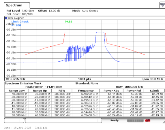
Plot on Channel 6515MHz 52RU40
