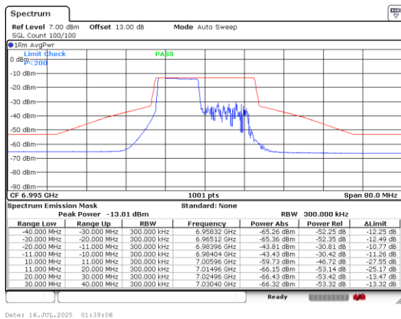
Plot on Channel 6995MHz 106RU53
