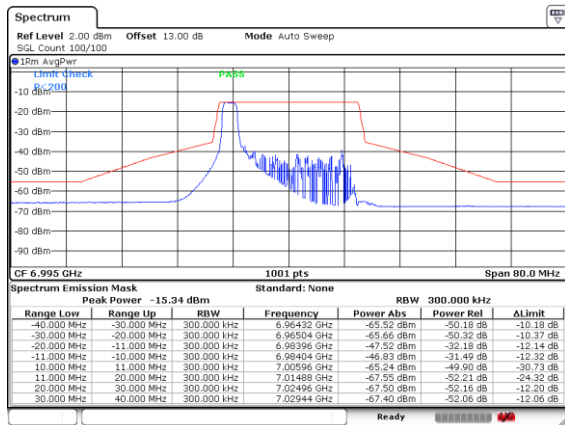
Plot on Channel 6995MHz 26RU0
