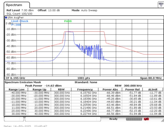
Plot on Channel 6195MHz 52RU37
