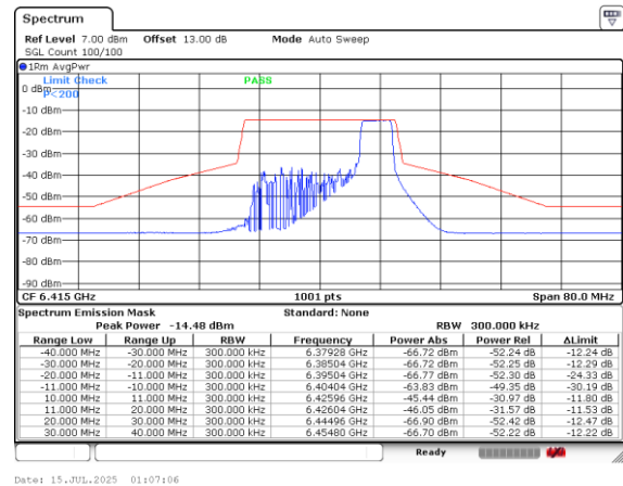
Plot on Channel 6415MHz 52RU40
