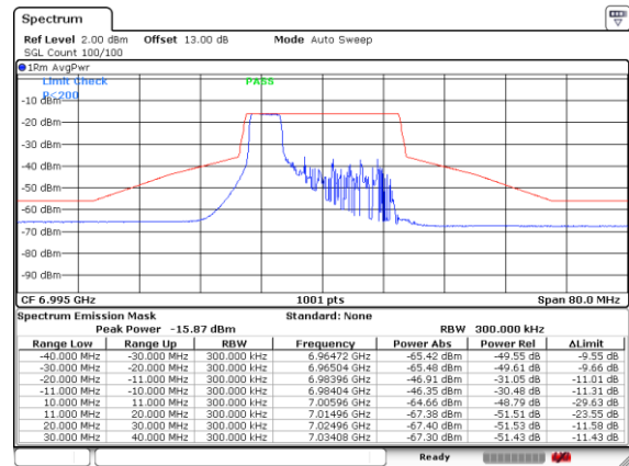
Plot on Channel 6995MHz 52RU37
