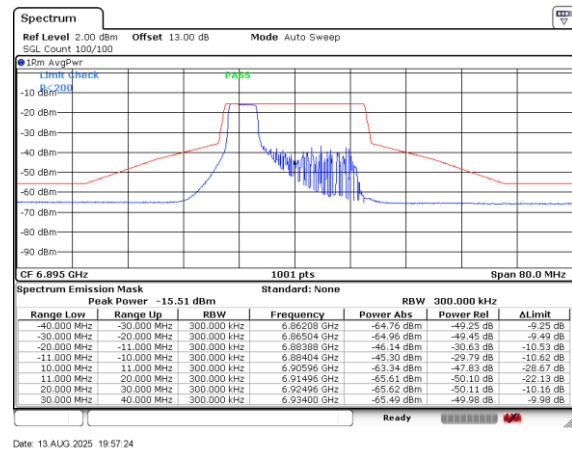
Plot on Channel 6895MHz 52RU37
