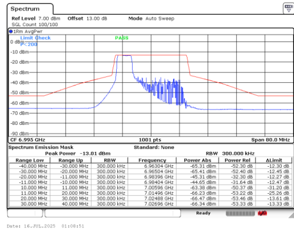
Plot on Channel 6995MHz 52RU37
