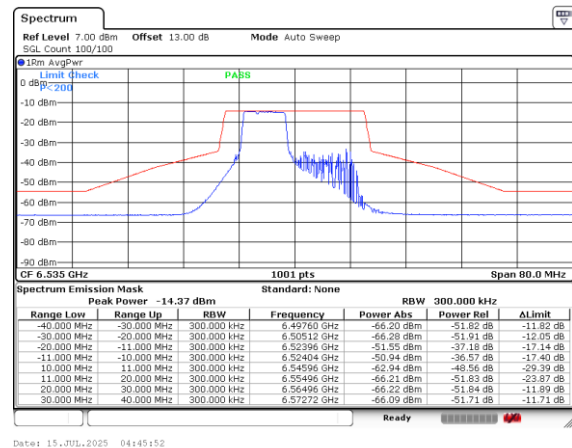
Plot on Channel 6535MHz Small RUs-52+2638
