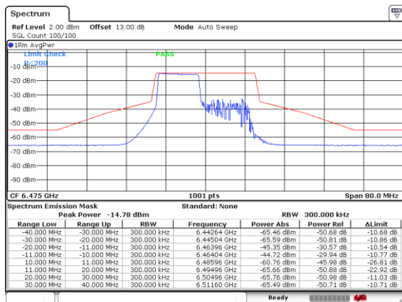
Plot on Channel 6475MHz 106RU53
