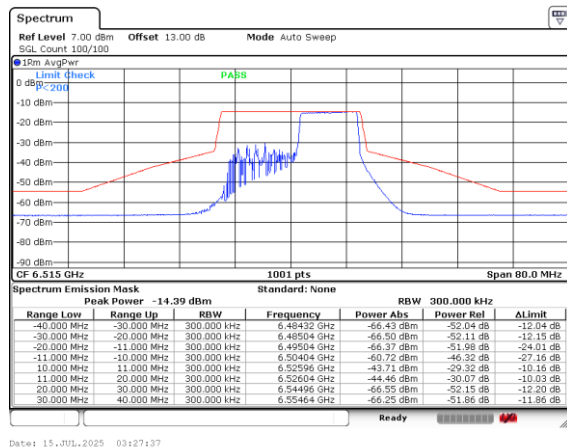
Plot on Channel 6515MHz 106RU54
