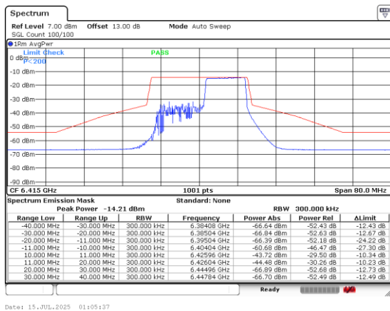
Plot on Channel 6415MHz 106RU54
