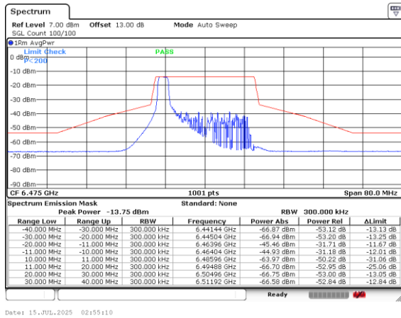
Plot on Channel 6475MHz 106RU53
