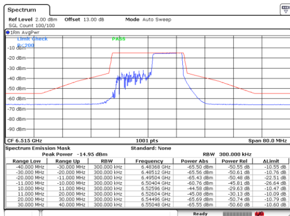
Plot on Channel 6515MHz 106RU54
