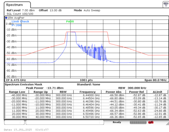
Plot on Channel 6475MHz 52RU37
