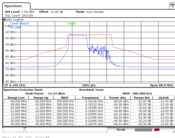
Plot on Channel 6195MHz 106RU53
