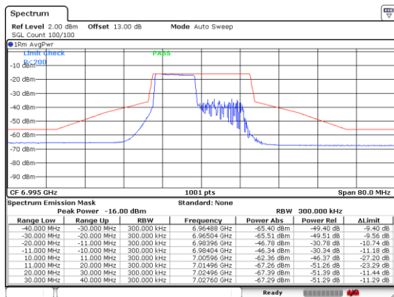
Plot on Channel 6995MHz 106RU53
