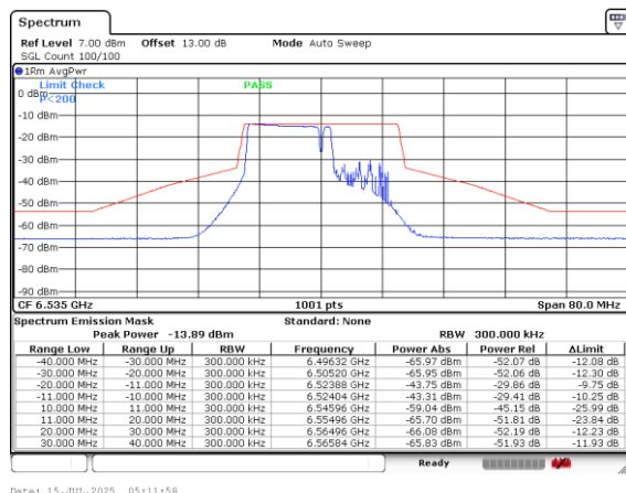
Plot on Channel 6535MHz Small RUs-106+2653
