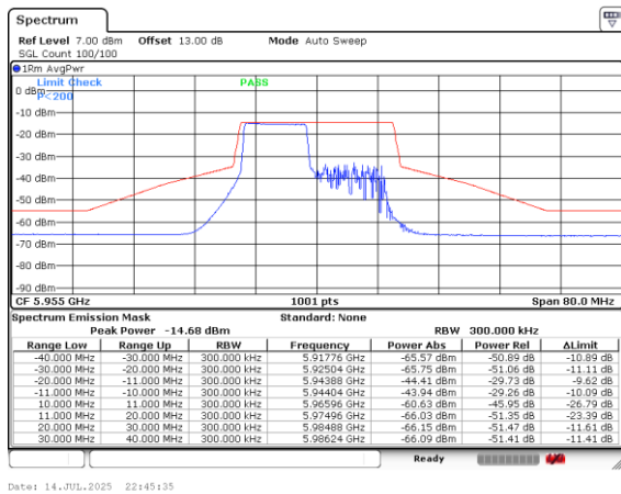
Plot on Channel 5955MHz Small RUs-106+2653
