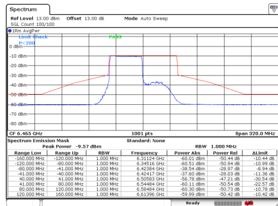
Plot on Channel 6465MHz 484RU65
