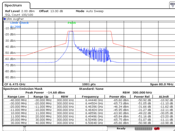
Plot on Channel 6475MHz 26RU0
