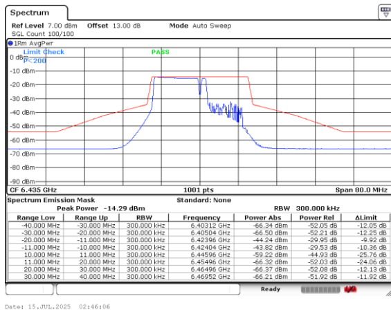
Plot on Channel 6435MHz Small RUs-106+2653
