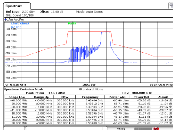
Plot on Channel 6515MHz 52RU40
