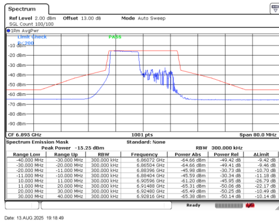
Plot on Channel 6895MHz 106RU53
