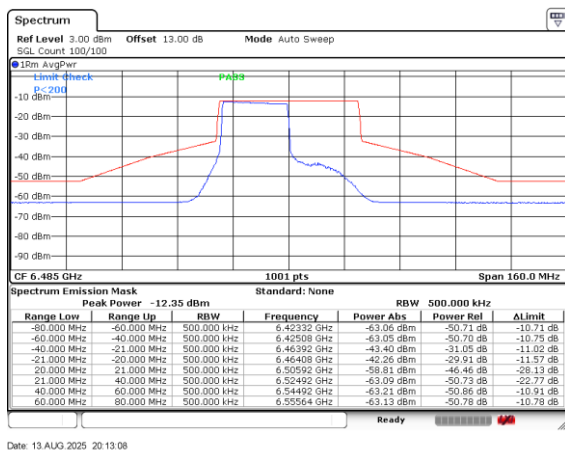
Plot on Channel 6485MHz 242RU61
