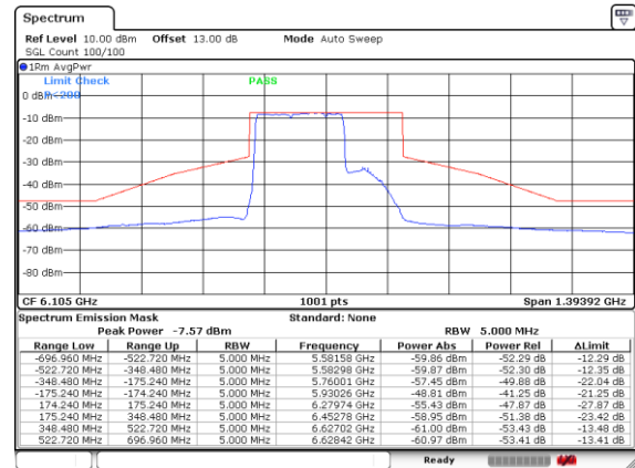
Plot on Channel 6105MHz Puncture 80+40M
