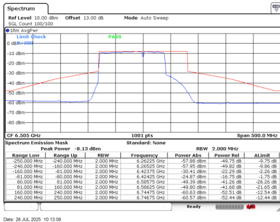
Plot on Channel 6505MHz Puncture 40M
