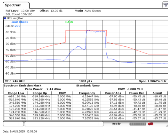
Plot on Channel 6745MHz Puncture 40M
