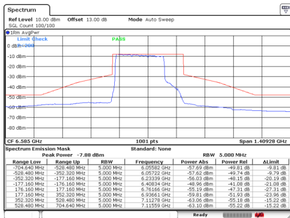
Plot on Channel 6585MHz Large RUs-996x3
