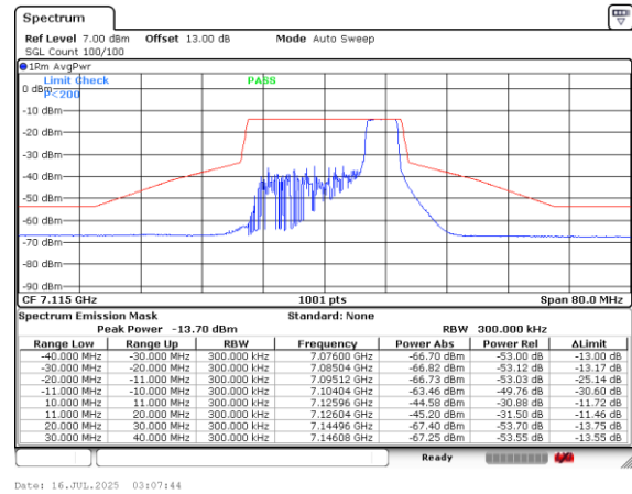
Plot on Channel 7115MHz Small RUs-52+2639
