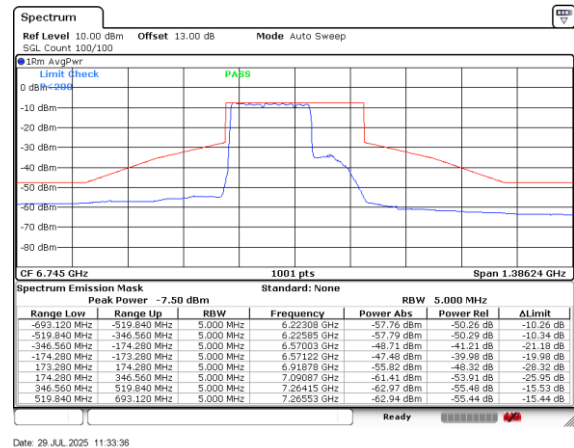
Plot on Channel 6745MHz Puncture 80+40M
