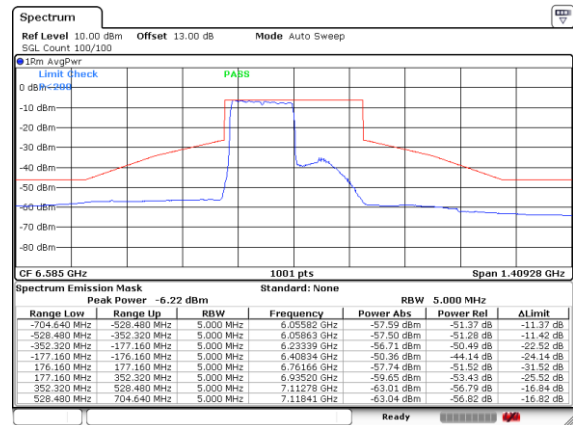
Plot on Channel 6585MHz 1992RU68
