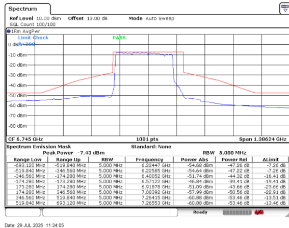
Plot on Channel 6745MHz Puncture 80M
