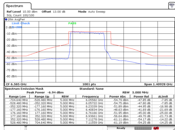
Plot on Channel 6585MHz Puncture 40M
