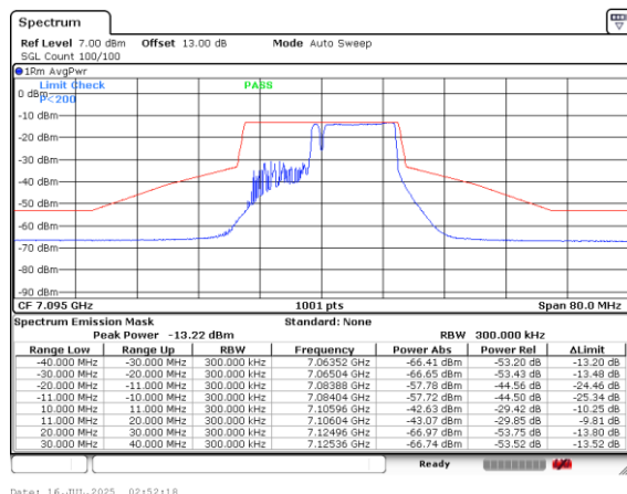
Plot on Channel 7095MHz Small RUs-106+2654
