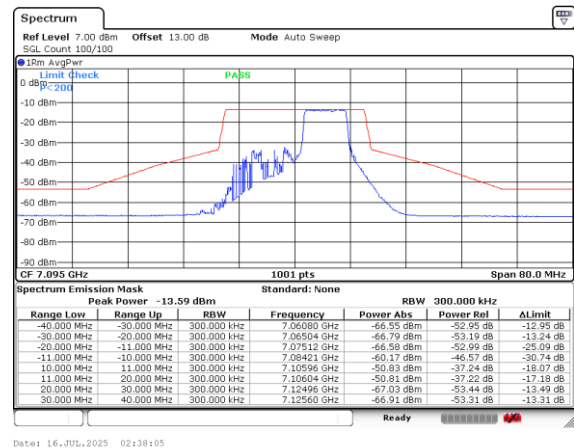
Plot on Channel 7095MHz Small RUs-52+2639
