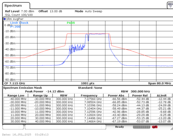
Plot on Channel 7115MHz Small RUs-106+2654
