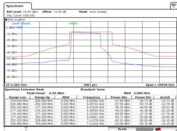
Plot on Channel 6585MHz Puncture 80M
