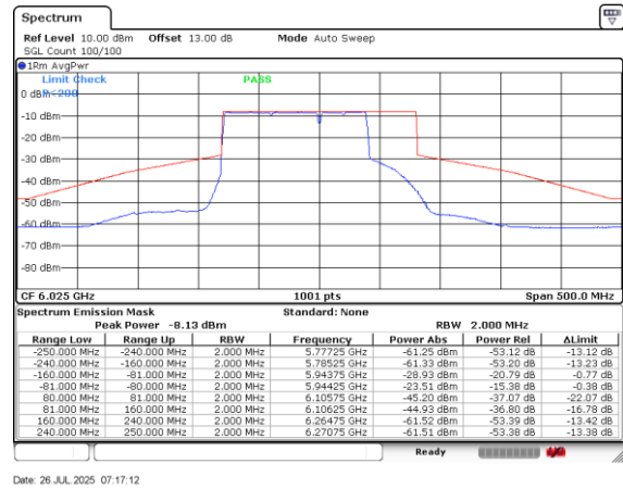
Plot on Channel 6025MHz Puncture 40M
