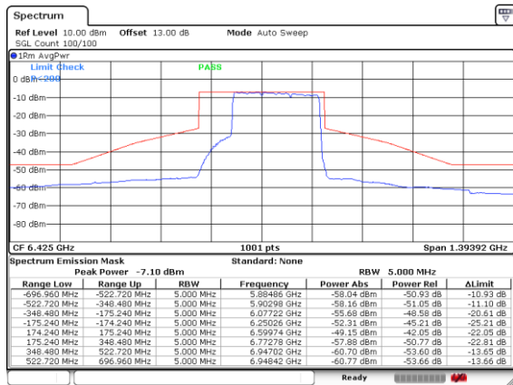
Plot on Channel 6425MHz Puncture 80M
