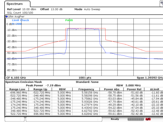
Plot on Channel 6105MHz Puncture 40M
