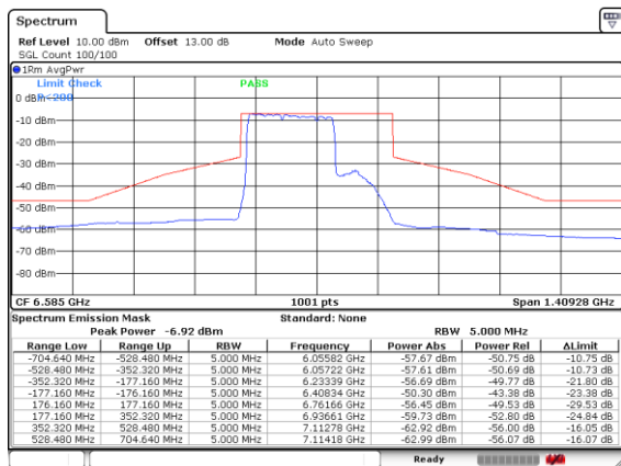
Plot on Channel 6585MHz Puncture 80+40M
