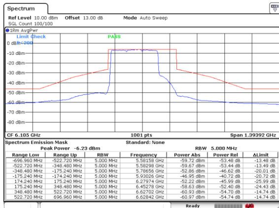
Plot on Channel 6105MHz Puncture 80M
