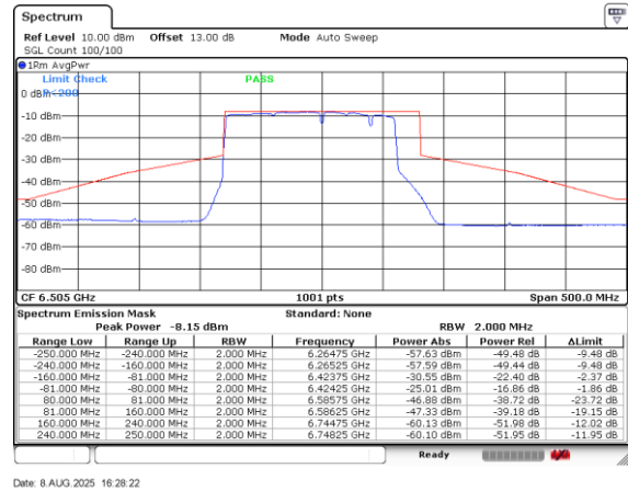
Plot on Channel 6505MHz Puncture 20M
