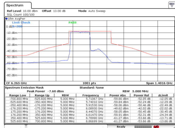
Plot on Channel 6265MHz 1992RU68
