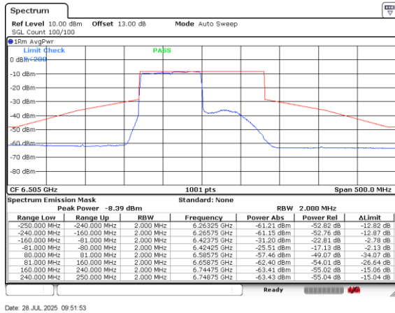
Plot on Channel 6505MHz Large RUs-996+484
