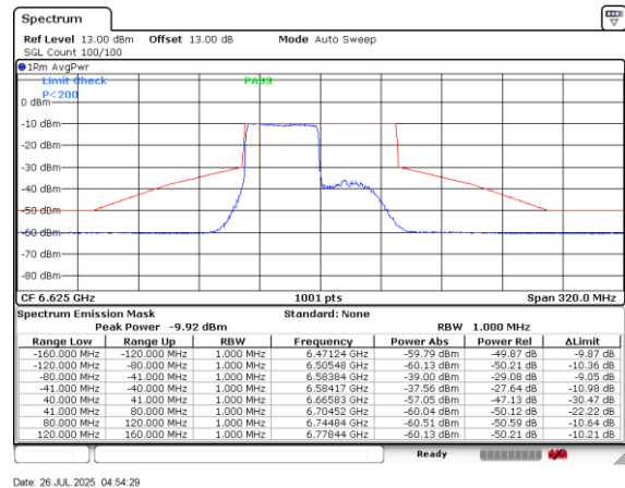
Plot on Channel 6625MHz Puncture 20M
