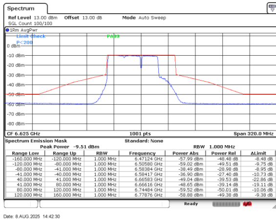
Plot on Channel 6625MHz _Large RUs-484+242
