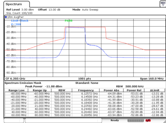
Plot on Channel 6205MHz 242RU61
