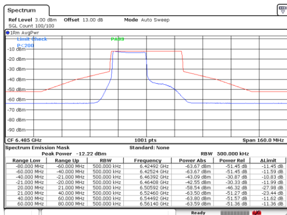
Plot on Channel 6485MHz 242RU61
