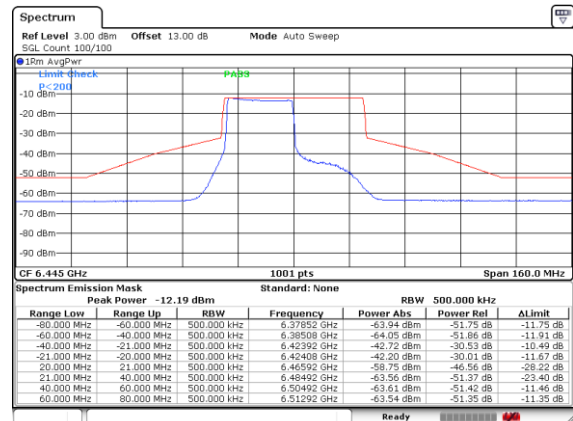
Plot on Channel 6445MHz 242RU61
