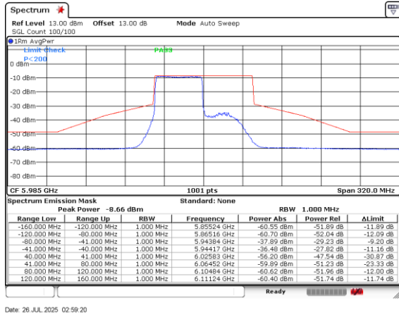
Plot on Channel 5985MHz Puncture 20M
