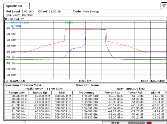
Plot on Channel 6525MHz 242RU62
