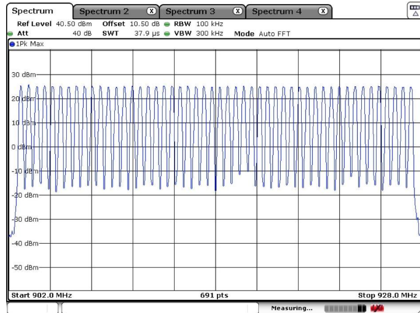
Number of Hopping Channel Plot
