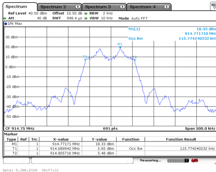
99% Occupied Bandwidth Plot on 914.75 MHz
