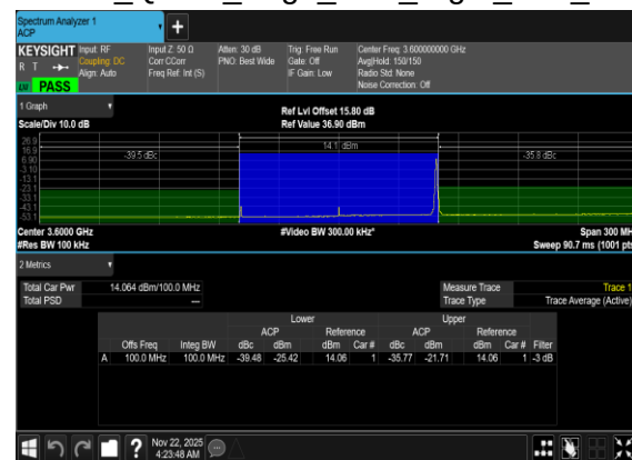
N77(100M)_DFT-s-OFDM_QPSK_Edge_1RB_Right_Low_CH
