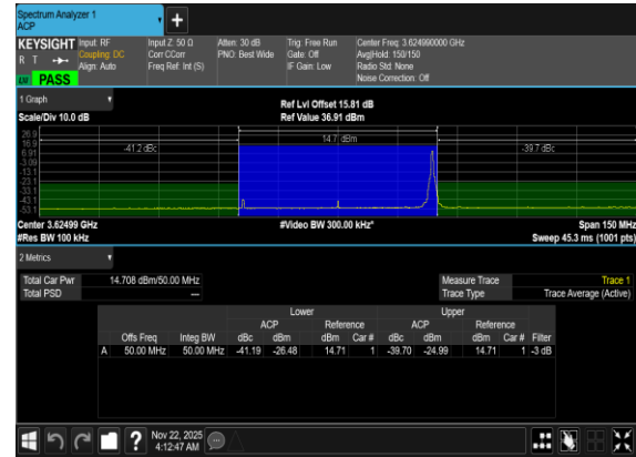
N77(50M)_DFT-s-OFDM_QPSK_Edge_1RB_Right_Mid_CH
