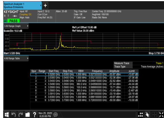
B5_N77(40M)_DFT-s-OFDM_QPSK_Edge_1RB_Right_Low_CH
