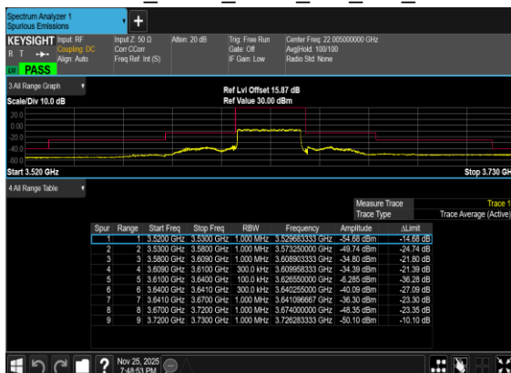
B5_N77(30M)_DFT-s- OFDM_BPSK_Outer_Full_Mid_CH
