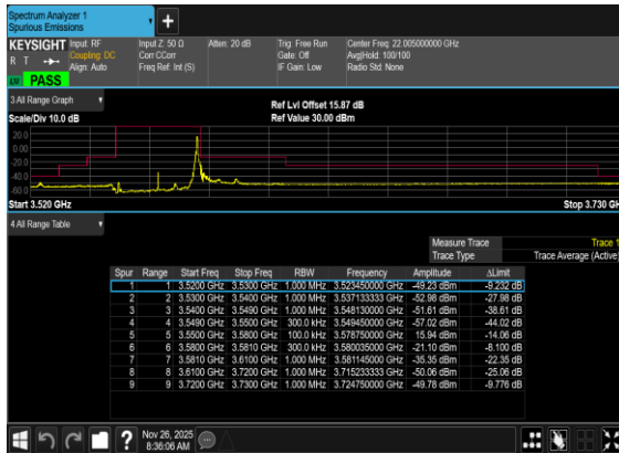
B5_N77(30M)_DFT-s- OFDM_BPSK_Edge_1RB_Right_Low_CH
