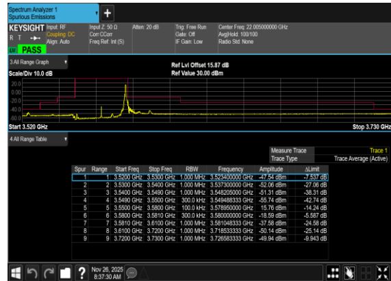
B5_N77(30M)_DFT-s- OFDM_QPSK_Edge_1RB_Right_Low_CH
