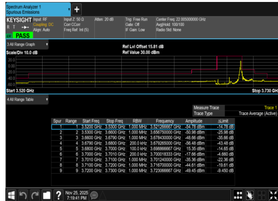
B5_N77(20M)_DFT-s-OFDM_QPSK_Edge_1RB_Right_High_CH
