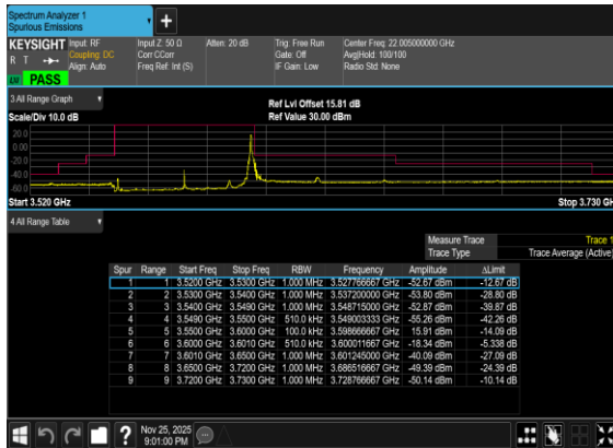
B5_N77(50M)_DFT-s- OFDM_BPSK_Edge_1RB_Right_Low_CH
