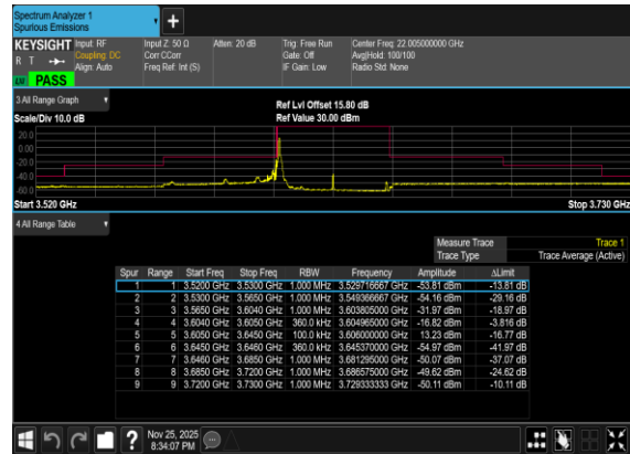
B5_N77(40M)_DFT-s-OFDM_QPSK_Edge_1RB_Left_Mid_CH
