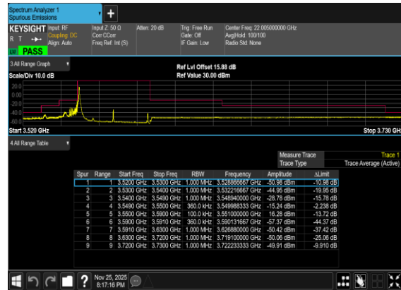
B5_N77(40M)_DFT-s-OFDM_QPSK_Edge_1RB_Left_Low_CH
