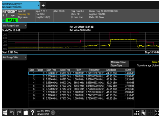
B5_N77(40M)_DFT-s- OFDM_BPSK_Outer_Full_High_CH
