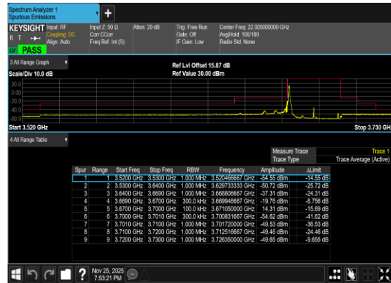
B5_N77(30M)_DFT-s- OFDM_BPSK_Edge_1RB_Left_High_CH
