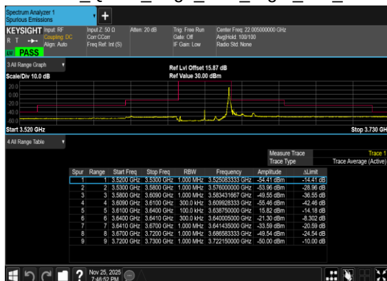
B5_N77(30M)_DFT-s- OFDM_QPSK_Edge_1RB_Right_Mid_CH
