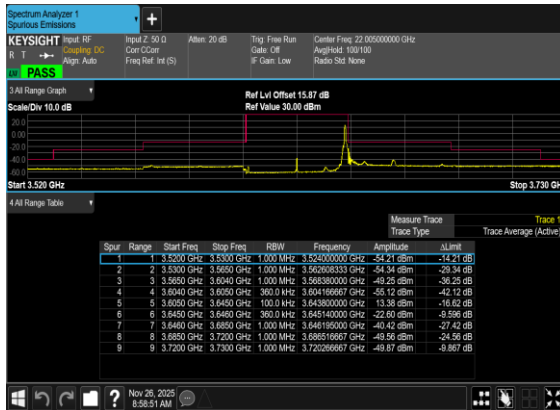
B5_N77(40M)_DFT-s-OFDM_BPSK_Edge_1RB_Right_Mid_CH
