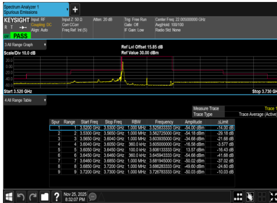
B5_N77(40M)_DFT-s-OFDM_BPSK_Edge_1RB_Left_Mid_CH
