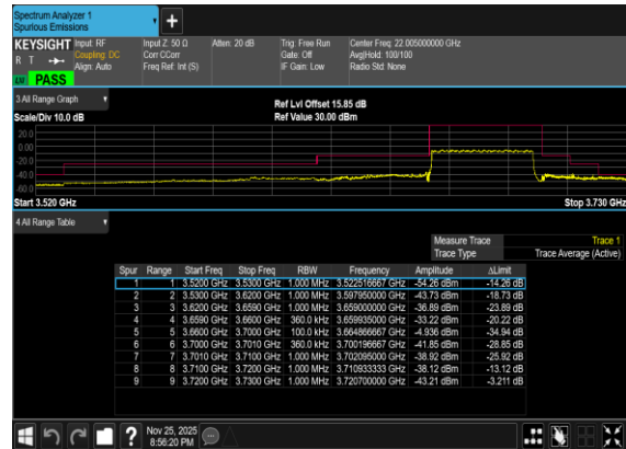
B5_N77(40M)_DFT-s- OFDM_QPSK_Outer_Full_High_CH
