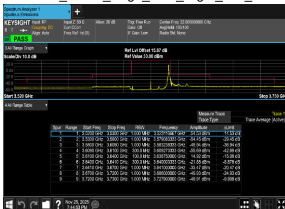
B5_N77(30M)_DFT-s- OFDM_BPSK_Edge_1RB_Right_Mid_CH
