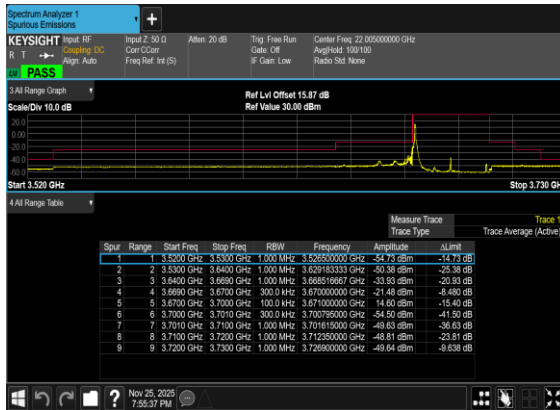
B5_N77(30M)_DFT-s- OFDM_QPSK_Edge_1RB_Left_High_CH
