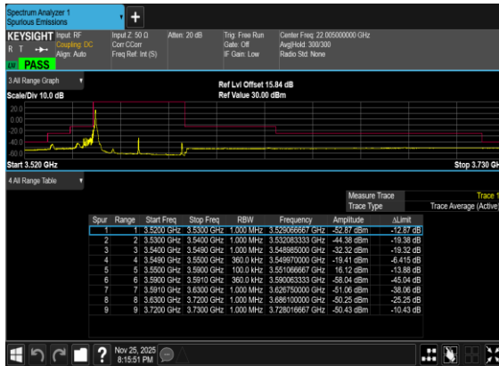
B5_N77(40M)_DFT-s-OFDM_BPSK_Edge_1RB_Left_Low_CH
