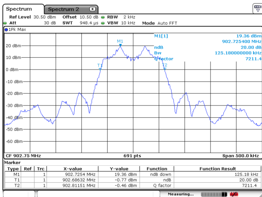
20 dB Bandwidth Plot on 902.75 MHz
