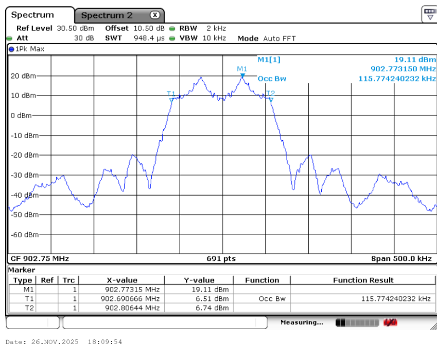
99% Occupied Bandwidth Plot on 902.75 MHz
