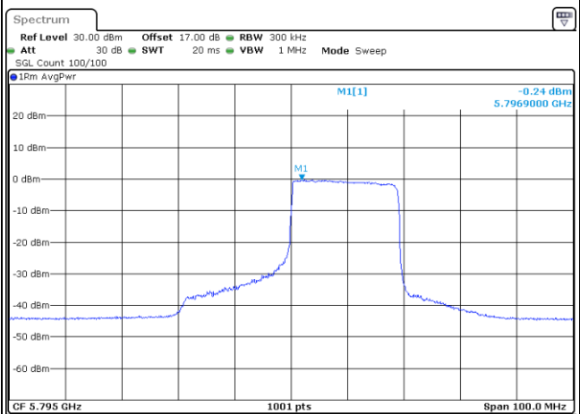
11AX40 5795MHz Partial RU242/62 MIMO Ant2
