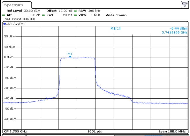
11AX40 5755MHz Partial RU242/61 MIMO Ant2
