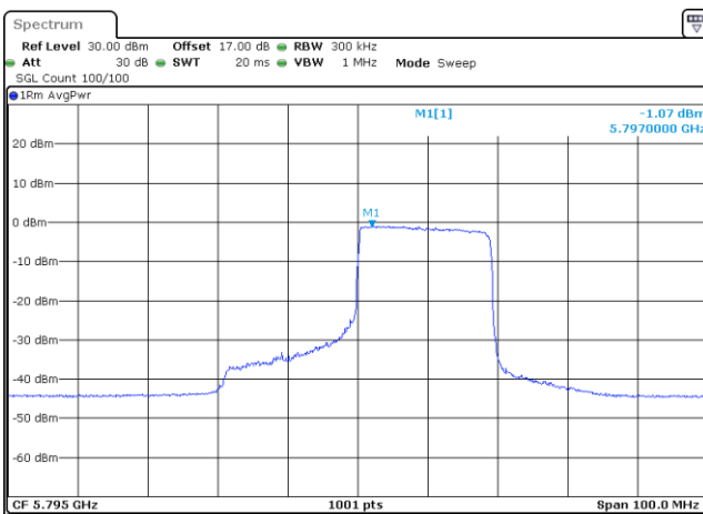
11AX40 5795MHz Partial RU242/62 MIMO Ant1
