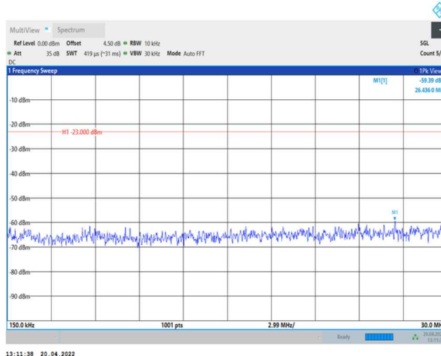
Band26-15MHz-QPSK-26865-1RB#0-Range2:0.15~30MHz
