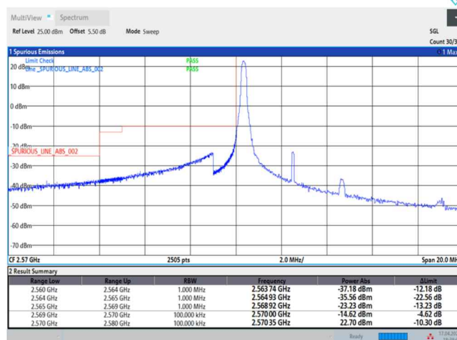
Band38-5MHz-QPSK-37775-25RB#0
