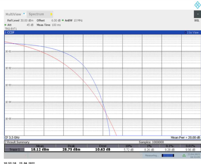
Band42-20MHz-QPSK-42590-100RB#0
