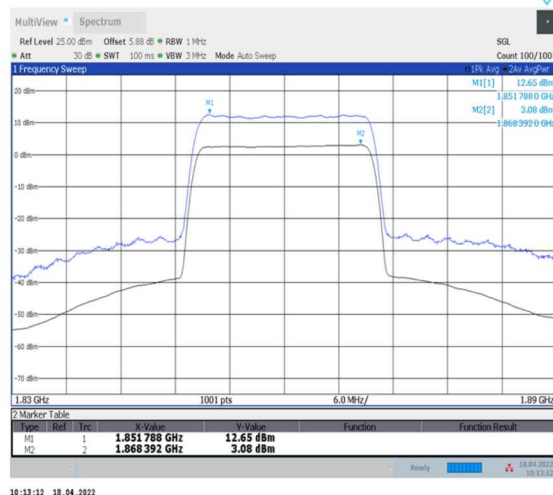
1-N2--15-20-L-2-CP-256QAM-Outer_Full-106@0- Ant0-9.57-100%-0.00-9.57-PASS-≤13
