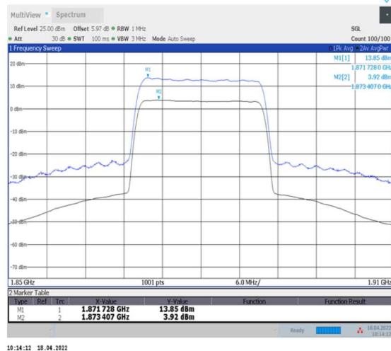
1-N2--15-20-M-2-CP-256QAM-Outer_Full-106@0- Ant0-9.93-100%-0.00-9.93-PASS-≤13
