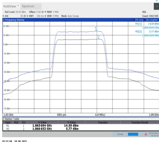
1-N2--15-20-L-1-DFT-256QAM-Outer_Full-100@0- Ant0-8.82-100%-0.00-8.82-PASS-≤13
