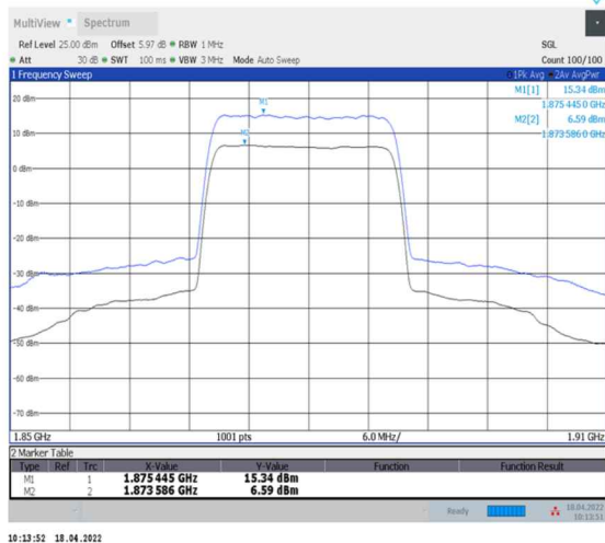
1-N2--15-20-M-1-DFT-256QAM-Outer_Full-100@0- Ant0-8.75-100%-0.00-8.75-PASS-≤13
