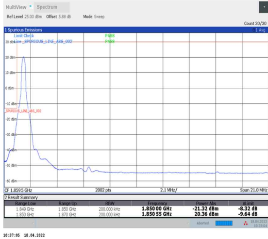
1-N2--15-20-L-1-DFT-PI2BPSK-Edge_1RB_Left-1@0-Ant0-seegraph-PASS-see graph
