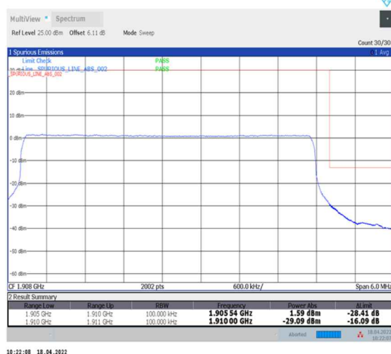
1-N2--15-5-H-6-CP-QPSK-Outer_Full-25@0-Ant0-seegraph-PASS-see graph
