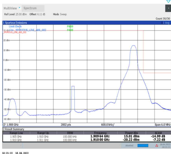
1-N2--15-5-H-5-CP-QPSK-Edge_1RB_Right-1@24-Ant0-seegraph-PASS-see graph
