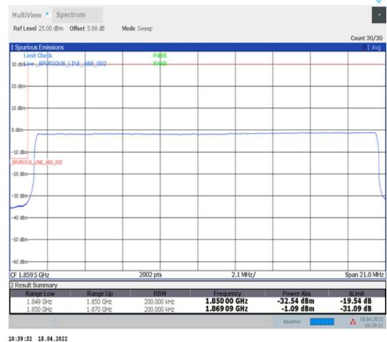
1-N2--15-20-L-6-CP-QPSK-Outer_Full-106@0-Ant0-seegraph-PASS-see graph
