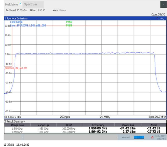
1-N2--15-20-L-3-DFT-PI2BPSK-Outer_Full-100@0-Ant0-seegraph-PASS-see graph
