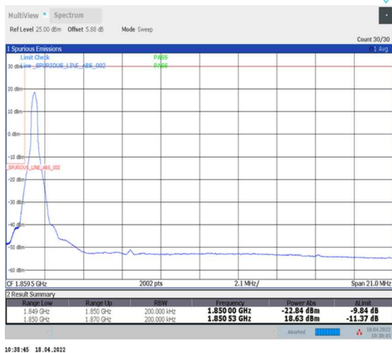
1-N2--15-20-L-4-CP-QPSK-Edge_1RB_Left-1@0-Ant0-seegraph-PASS-see graph
