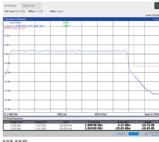
1-N2--15-5-H-3-DFT-PI2BPSK-Outer_Full-25@0-Ant0-seegraph-PASS-see graph
