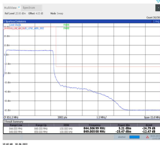
1-N5--15-5-H-6-CP-QPSK-Outer_Full-25@0-Ant0-seegraph-PASS-see graph
