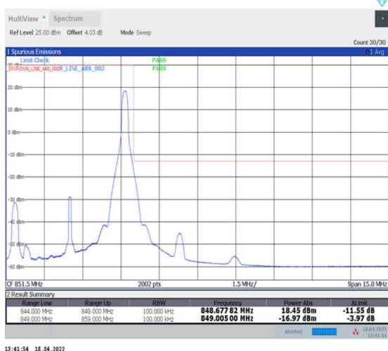
1-N5--15-5-H-5-CP-QPSK-Edge_1RB_Right-1@24-Ant0-seegraph-PASS-see graph
