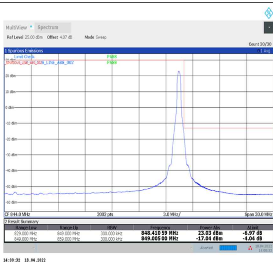
1-N5--15-20-H-2-DFT-PI2BPSK-Edge_1RB_Right-1@105-Ant0-seegraph-PASS-see graph
