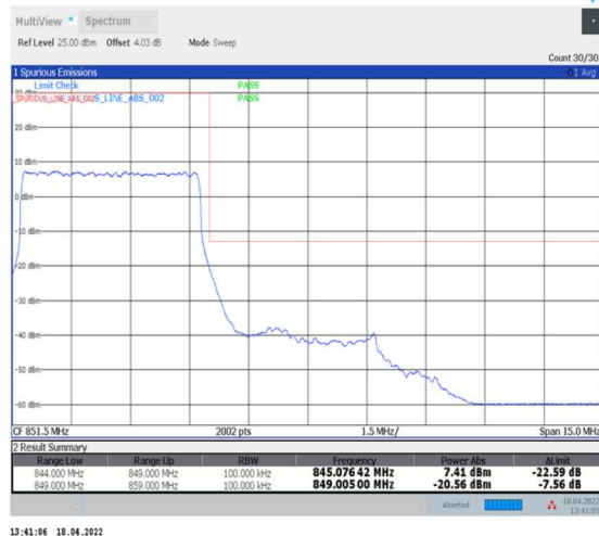
1-N5--15-5-H-3-DFT-PI2BPSK-Outer_Full-25@0-Ant0-seegraph-PASS-see graph
