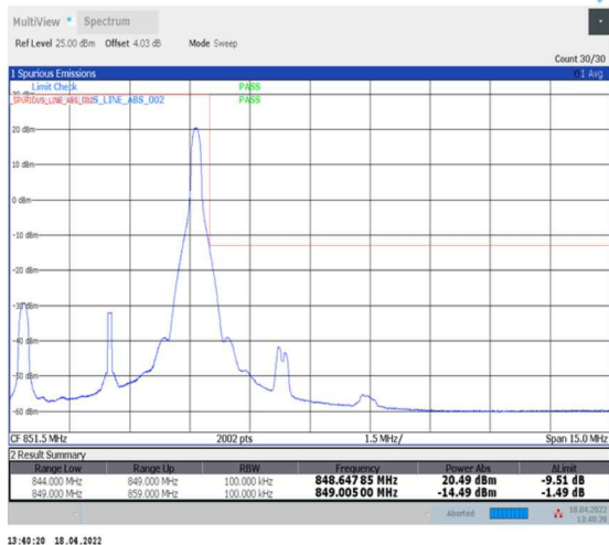
1-N5--15-5-H-2-DFT-PI2BPSK-Edge_1RB_Right-1@24-Ant0-seegraph-PASS-see graph
