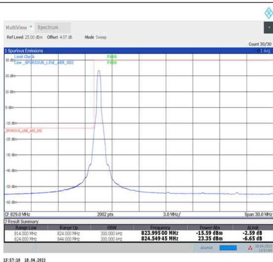
1-N5--15-20-L-1-DFT-PI2BPSK-Edge_1RB_Left-1@0-Ant0-seegraph-PASS-see graph
