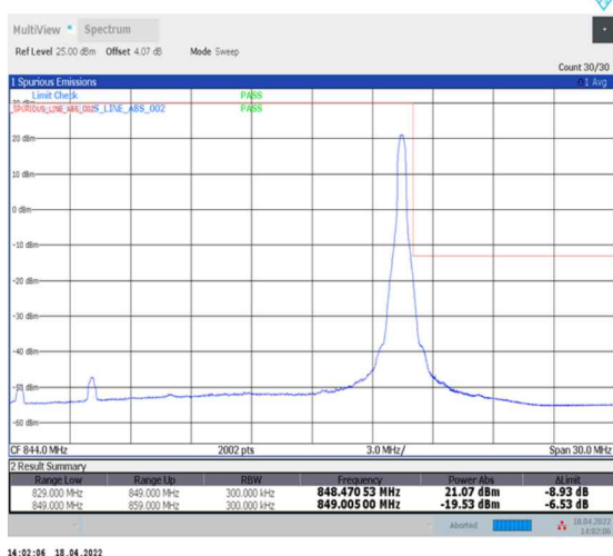
1-N5--15-20-H-5-CP-QPSK-Edge_1RB_Right-1@105-Ant0-seegraph-PASS-see graph
