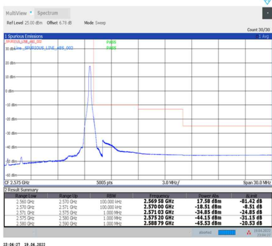
1-N7--15-10-H-5-CP-QPSK-Edge_1RB_Right-1@51-Ant0-PASS-see graph
