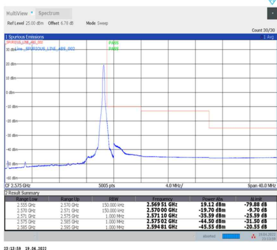
1-N7--15-15-H-5-CP-QPSK-Edge_1RB_Right-1@78-Ant0-PASS-see graph
