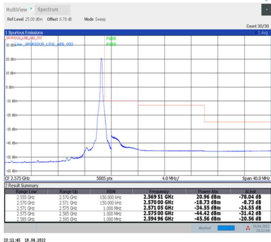
1-N7--15-15-H-2-DFT-PI2BPSK-Edge_1RB_Right-1@78-Ant0-PASS-see graph
