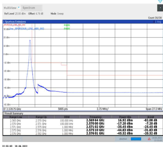
1-N7--15-5-H-5-CP-QPSK-Edge_1RB_Right-1@24-Ant0-PASS-see graph
