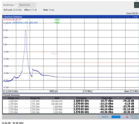
1-N7--15-5-H-2-DFT-PI2BPSK-Edge_1RB_Right-1@24-Ant0-PASS-see graph
