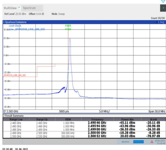
1-N7--15-20-L-4-CP-QPSK-Edge_1RB_Left-1@0-Ant0-PASS-see graph
