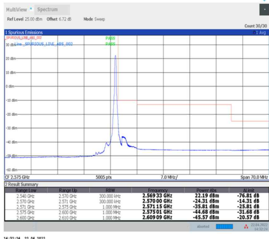
1-N7--15-30-H-2-DFT-PI2BPSK-Edge_1RB_Right-1@159-Ant0-PASS-see graph
