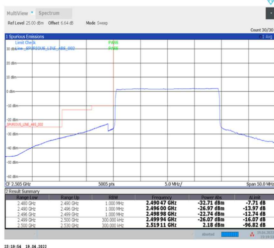
1-N7--15-20-L-6-CP-QPSK-Outer_Full-106@0-Ant0-PASS-see graph
