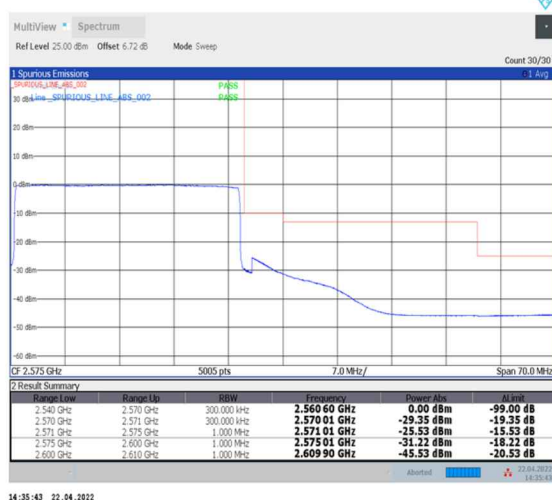
1-N7--15-30-H-6-CP-QPSK-Outer_Full-160@0-Ant0-PASS-see graph
