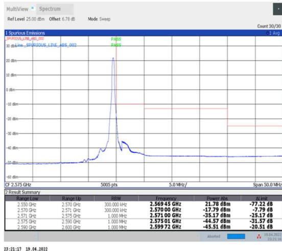
1-N7--15-20-H-2-DFT-PI2BPSK-Edge_1RB_Right-1@105-Ant0-PASS-see graph
