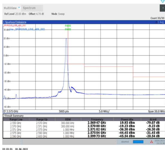
1-N7--15-20-H-5-CP-QPSK-Edge_1RB_Right-1@105-Ant0-PASS-see graph
