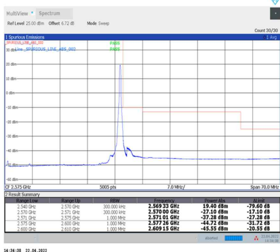
1-N7--15-30-H-5-CP-QPSK-Edge_1RB_Right-1@159-Ant0-PASS-see graph
