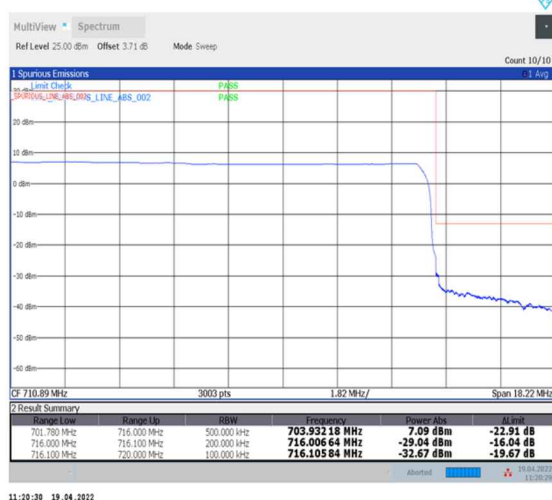
1-N12--15-15-H-6-CP-QPSK-Outer_Full-79@0-Ant0-PASS-see graph
