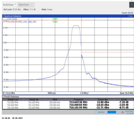
1-N12--15-10-H-2-DFT-PI2BPSK-Edge_1RB_Right-1@51-Ant0-PASS-see graph
