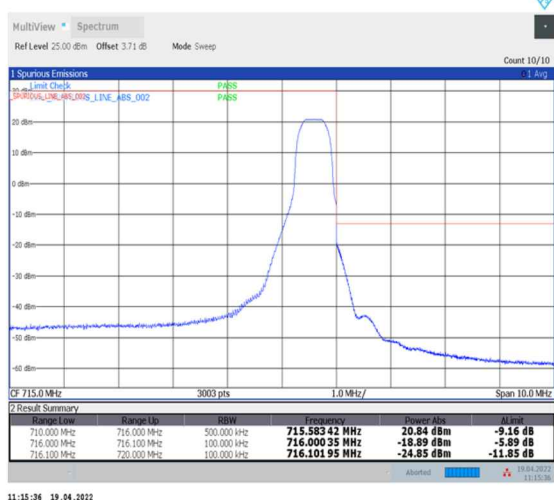
1-N12--15-10-H-5-CP-QPSK-Edge_1RB_Right-1@51-Ant0-PASS-see graph
