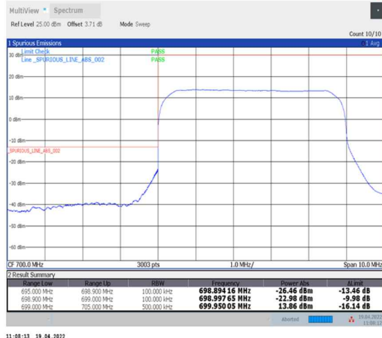
1-N12--15-5-L-3-DFT-PI2BPSK-Outer_Full-25@0-Ant0-PASS-see graph
