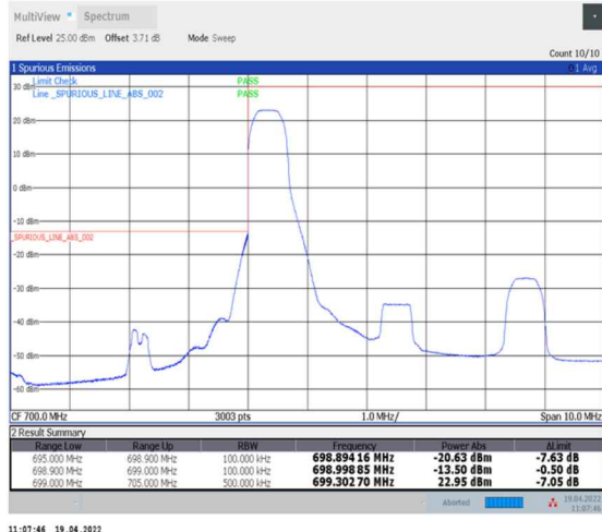
1-N12--15-5-L-1-DFT-PI2BPSK-Edge_1RB_Left-1@0-Ant0-PASS-see graph
