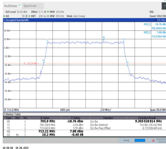
1-N12--15-10-H-9-CP-256QAM-Outer_Full-52@0-Ant0-9.305-10.200-≤10-PASS
