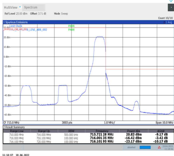
1-N12--15-5-H-5-CP-QPSK-Edge_1RB_Right-1@24-Ant0-PASS-see graph
