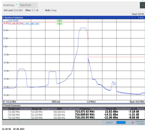
1-N12--15-5-H-2-DFT-PI2BPSK-Edge_1RB_Right-1@24-Ant0-PASS-see graph
