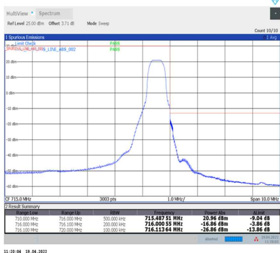
1-N12--15-15-H-5-CP-QPSK-Edge_1RB_Right-1@78-Ant0-PASS-see graph
