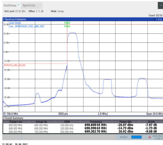
1-N12--15-5-L-4-CP-QPSK-Edge_1RB_Left-1@0-Ant0-PASS-see graph
