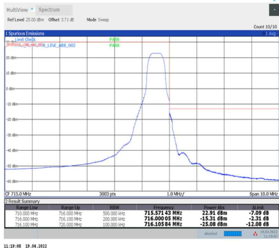
1-N12--15-15-H-2-DFT-PI2BPSK-Edge_1RB_Right-1@78-Ant0-PASS-see graph
