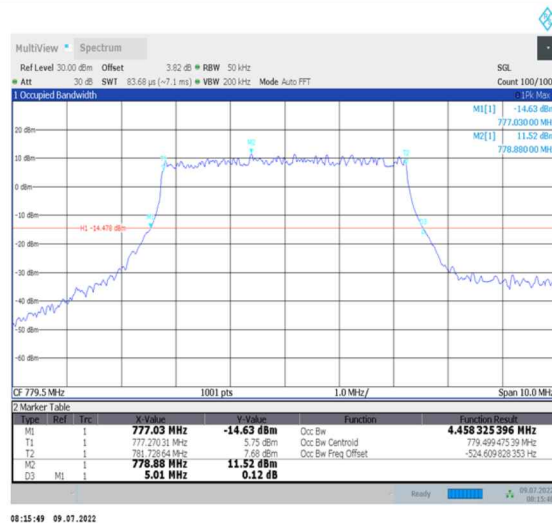
1-N13--15-5-L-4-DFT-64QAM-Outer_Full-25@0-Ant0-4.458-5.010-≤5-PASS
