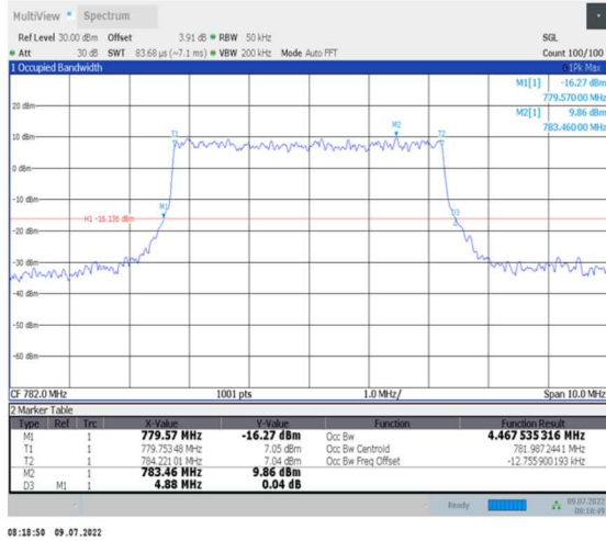
1-N13--15-5-M-8-CP-64QAM-Out Full-25@0-Ant0-4.468-4.880-≤5-PASS
