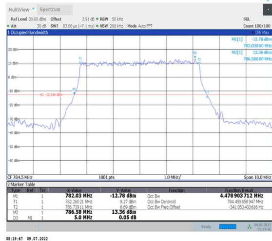
1-N13--15-5-H-2-DFT-PI2BPSK-Out Full-25@0-Ant0-4.479-5.000-≤5-PASS
