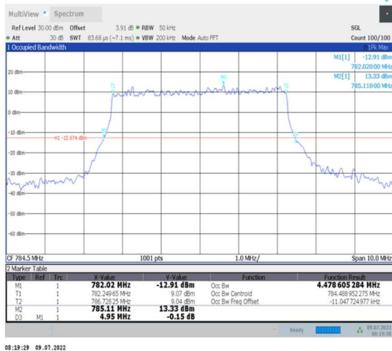
1-N13--15-5-H-1-DFT-QPSK-Out Full-25@0-Ant0-4.479-4.950-≤5-PASS
