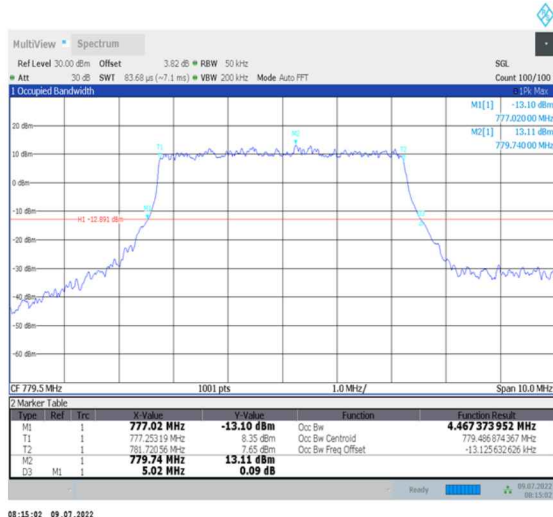
1-N13--15-5-L-1-DFT-QPSK-Outer_Full-25@0-Ant0-4.467-5.020-≤5-PASS
