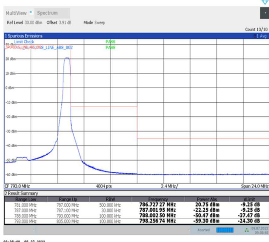
1-N13-PC3-15-5-H-5-CP-QPSK-Edge_1RB_Right-1@24-Ant0-PASS-see graph
