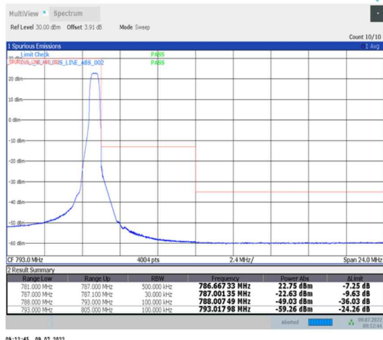
1-N13-PC3-15-10-H-2-DFT-PI2BPSK-Edge_1RB_Right-1@51-Ant0-PASS-see graph
