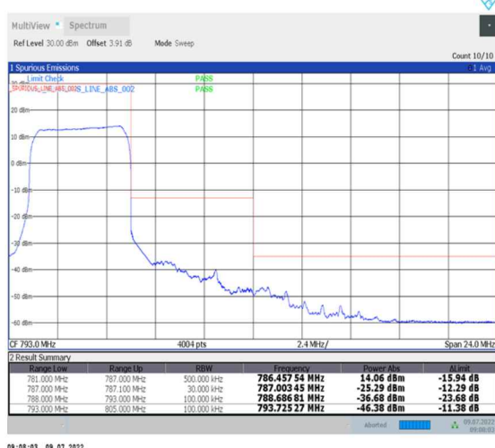
1-N13-PC3-15-5-H-3-DFT-PI2BPSK-Outer_Full-25@0-Ant0-PASS-see graph
