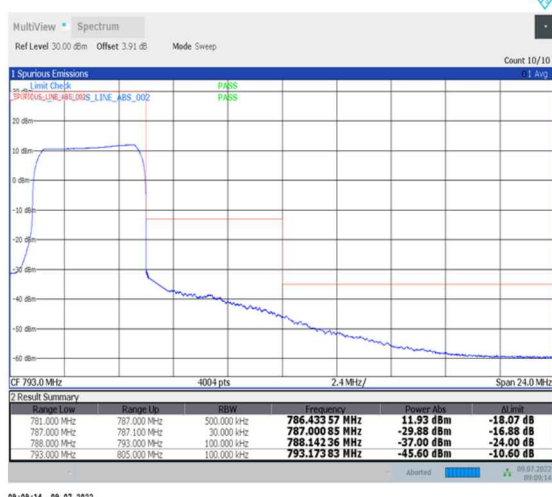
1-N13-PC3-15-5-H-6-CP-QPSK-Outer_Full-25@0-Ant0-PASS-see graph
