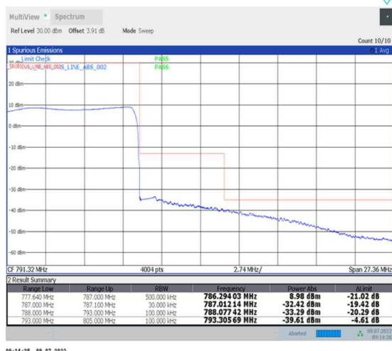
1-N13-PC3-15-10-H-6-CP-QPSK-Outer_Full-52@0-Ant0-PASS-see graph
