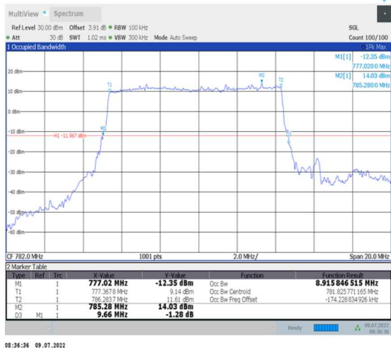
1-N13--15-10-M-2-DFT-PI2BPSK-Outer_Full-50@0-Ant0-8.916-9.660-≤10-PASS
