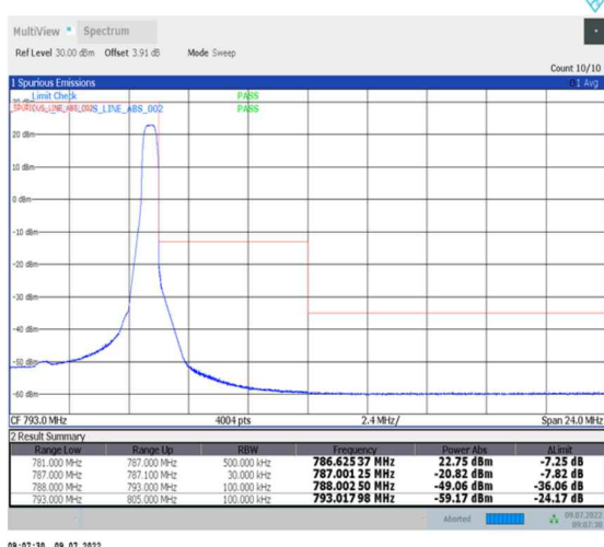
1-N13-PC3-15-5-H-2-DFT-PI2BPSK-Edge_1RB_Right-1@24-Ant0-PASS-see graph
