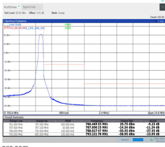
1-N13-PC3-15-10-H-5-CP-QPSK-Edge_1RB_Right-1@51-Ant0-PASS-see graph
