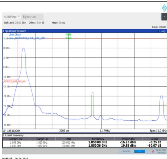
1-N25--15-10-L-1-DFT-PI2BPSK-Edge_1RB_Left-1@0-Ant0-seegraph-PASS-see graph
