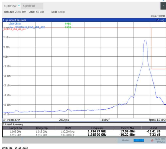
1-N25--15-10-H-2-DFT-PI2BPSK-Edge_1RB_Right-1@51-Ant0-seegraph-PASS-see graph
