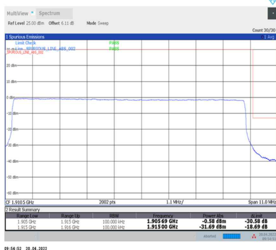
1-N25--15-10-H-6-CP-QPSK-Outer_Full-52@0-Ant0-seegraph-PASS-see graph
