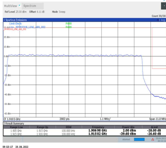
1-N25--15-10-H-3-DFT-PI2BPSK-Outer_Full-50@0-Ant0-seegraph-PASS-see graph
