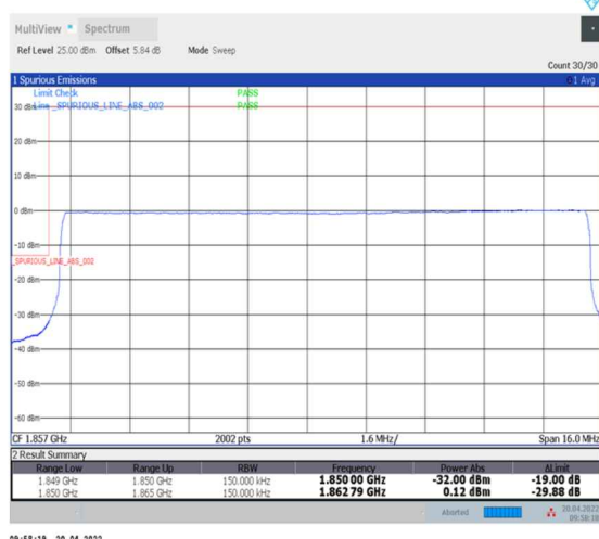
1-N25--15-15-L-6-CP-QPSK-Outer_Full-79@0-Ant0-seegraph-PASS-see graph
