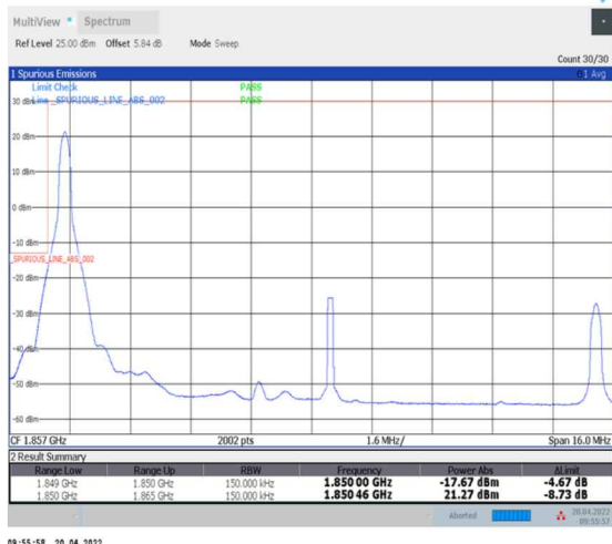
1-N25--15-15-L-1-DFT-PI2BPSK-Edge_1RB_Left-1@0-Ant0-seegraph-PASS-see graph
