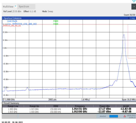
1-N25--15-15-H-5-CP-QPSK-Edge_1RB_Right-1@78-Ant0-seegraph-PASS-see graph
