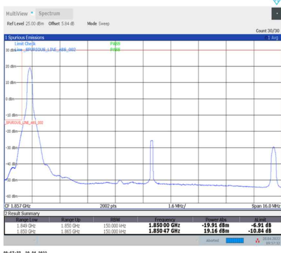
1-N25--15-15-L-4-CP-QPSK-Edge_1RB_Left-1@0-Ant0-seegraph-PASS-see graph
