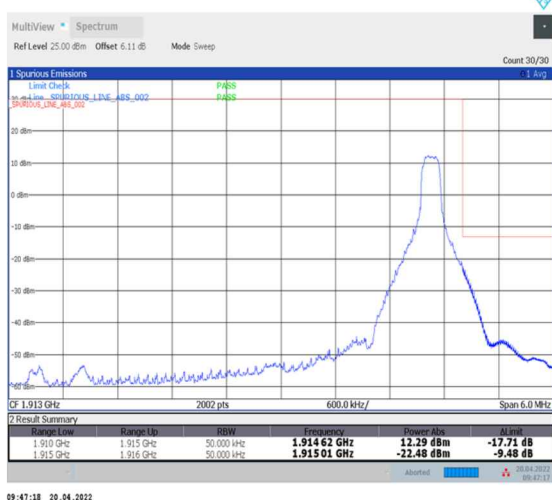
1-N25--15-5-H-5-CP-QPSK-Edge_1RB_Right-1@24-Ant0-seegraph-PASS-see graph
