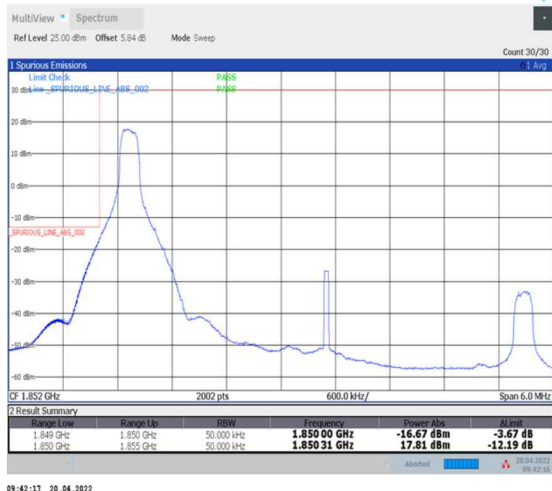
1-N25--15-5-L-1-DFT-PI2BPSK-Edge_1RB_Left-1@0-Ant0-seegraph-PASS-see graph
