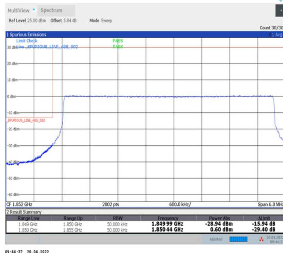
1-N25--15-5-L-6-CP-QPSK-Outer_Full-25@0-Ant0-seegraph-PASS-see graph
