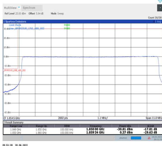
1-N25--15-10-L-6-CP-QPSK-Outer_Full-52@0-Ant0-seegraph-PASS-see graph
