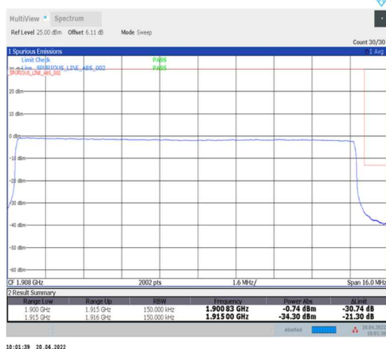
1-N25--15-15-H-6-CP-QPSK-Outer_Full-79@0-Ant0-seegraph-PASS-see graph
