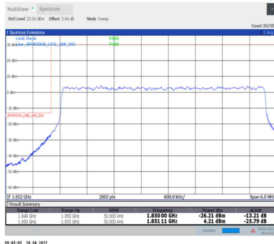
1-N25--15-5-L-3-DFT-PI2BPSK-Outer_Full-25@0-Ant0-seegraph-PASS-see graph
