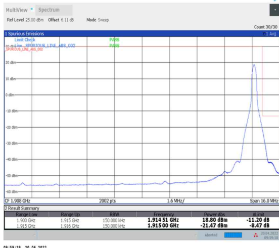
1-N25--15-15-H-2-DFT-PI2BPSK-Edge_1RB_Right-1@78-Ant0-seegraph-PASS-see graph
