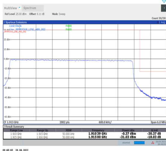
1-N25--15-5-H-6-CP-QPSK-Outer_Full-25@0-Ant0-seegraph-PASS-see graph
