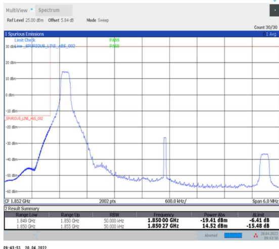
1-N25--15-5-L-4-CP-QPSK-Edge_1RB_Left-1@0-Ant0-seegraph-PASS-see graph
