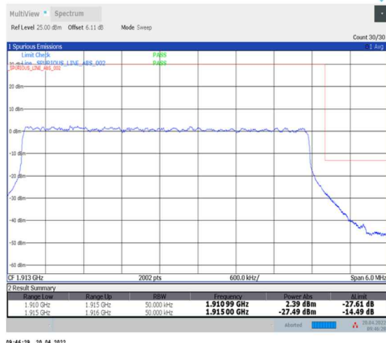
1-N25--15-5-H-3-DFT-PI2BPSK-Outer_Full-25@0-Ant0-seegraph-PASS-see graph
