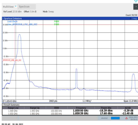
1-N25--15-10-L-4-CP-QPSK-Edge_1RB_Left-1@0-Ant0-seegraph-PASS-see graph
