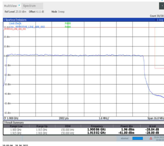
1-N25--15-15-H-3-DFT-PI2BPSK-Outer_Full-75@0-Ant0-seegraph-PASS-see graph
