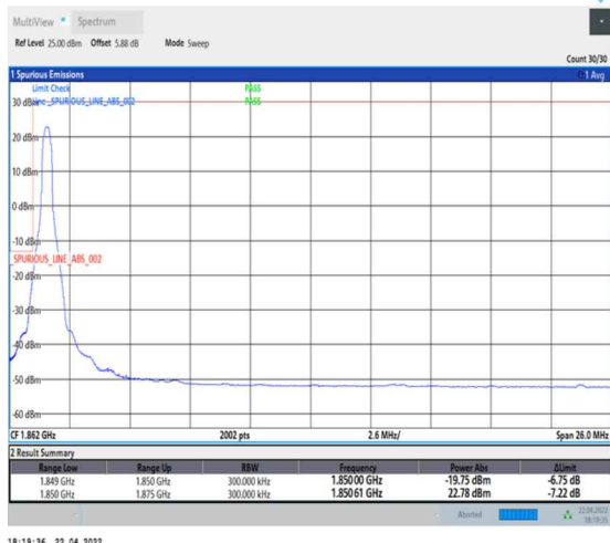
1-N25--15-25-L-1-DFT-PI2BPSK-Edge_1RB_Left-1@0-Ant0-seegraph-PASS-see graph
