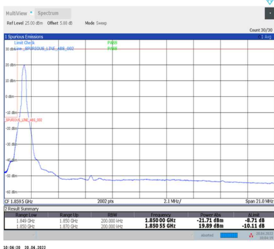
1-N25--15-20-L-4-CP-QPSK-Edge_1RB_Left-1@0-Ant0-seegraph-PASS-see graph
