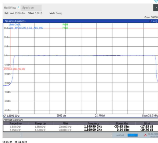
1-N25--15-20-L-6-CP-QPSK-Outer_Full-106@0-Ant0-seegraph-PASS-see graph
