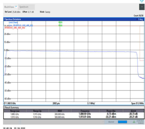
1-N25--15-30-H-6-CP-QPSK-Outer_Full-160@0-Ant0-seegraph-PASS-see graph
