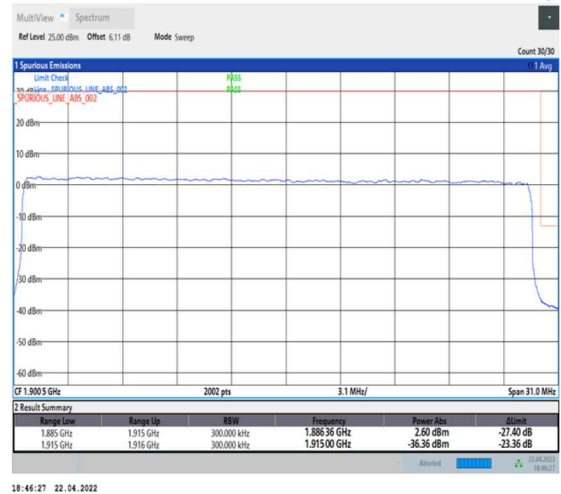
1-N25--15-30-H-3-DFT-PI2BPSK-Outer_Full-160@0-Ant0-seegraph-PASS-see graph
