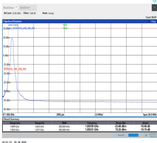
1-N25--15-25-L-4-CP-QPSK-Edge_1RB_Left-1@0-Ant0-seegraph-PASS-see graph
