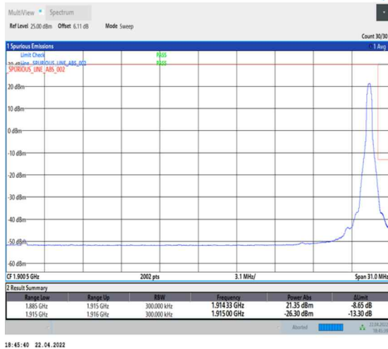
1-N25--15-30-H-2-DFT-PI2BPSK-Edge_1RB_Right-1@159-Ant0-seegraph-PASS-see graph
