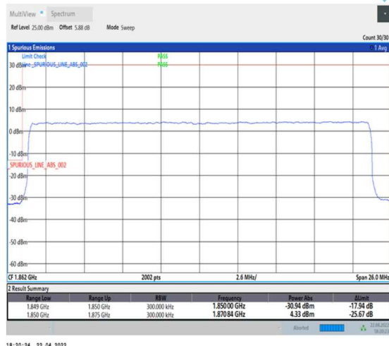
1-N25--15-25-L-3-DFT-PI2BPSK-Outer_Full-128@0-Ant0-seegraph-PASS-see graph
