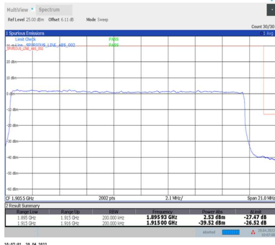
1-N25--15-20-H-3-DFT-PI2BPSK-Outer_Full-100@0-Ant0-seegraph-PASS-see graph
