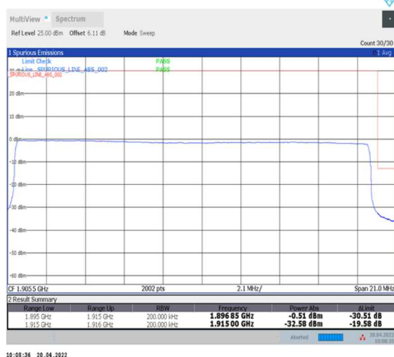
1-N25--15-20-H-6-CP-QPSK-Outer_Full-106@0-Ant0-seegraph-PASS-see graph
