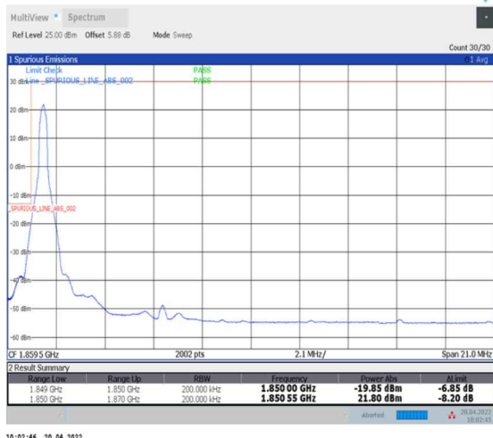
1-N25--15-20-L-1-DFT-PI2BPSK-Edge_1RB_Left-1@0-Ant0-seegraph-PASS-see graph
