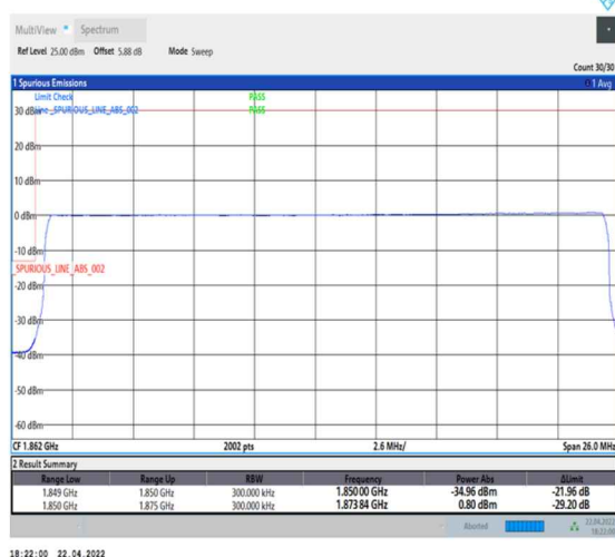
1-N25--15-25-L-6-CP-QPSK-Outer_Full-133@0-Ant0-seegraph-PASS-see graph
