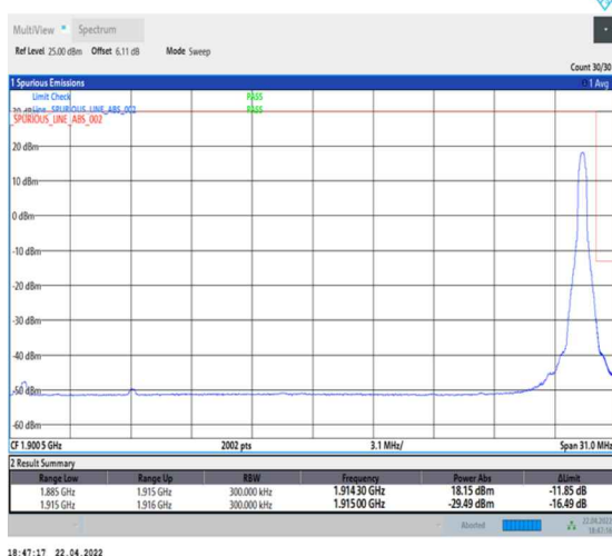
1-N25--15-30-H-5-CP-QPSK-Edge_1RB_Right-1@159-Ant0-seegraph-PASS-see graph
