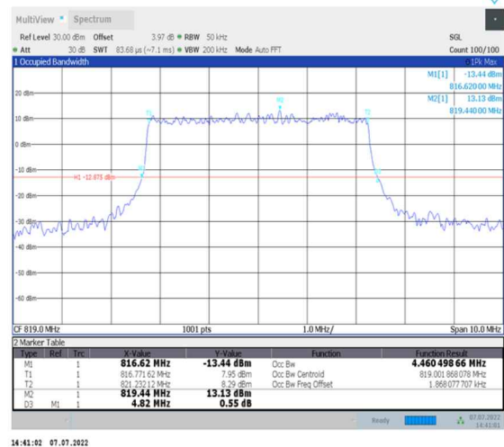
1-N26-814-824--15-5-M-3-DFT-16QAM-Outer_Full-25@0-Ant0-4.46-4.820-≤5-PASS
