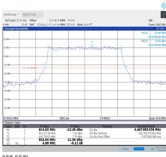
1-N26-814-824--15-5-L-3-DFT-16QAM-Outer_Full-25@0-Ant0-4.468-4.980-≤5-PASS
