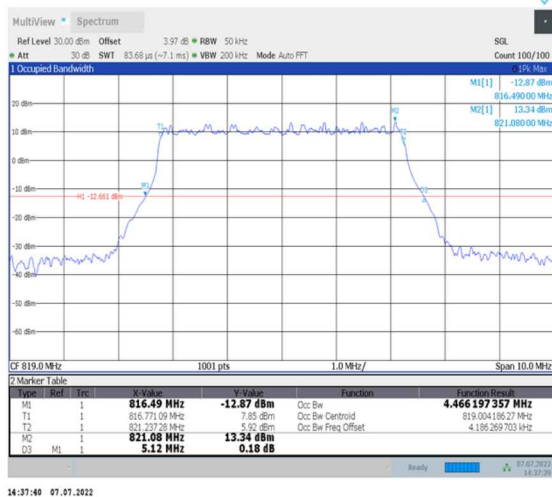
1-N26-814-824--15-5-M-2-DFT-PI2BPSK-Outer_Full-25@0-Ant0-4.466-5.120-≤5-PASS
