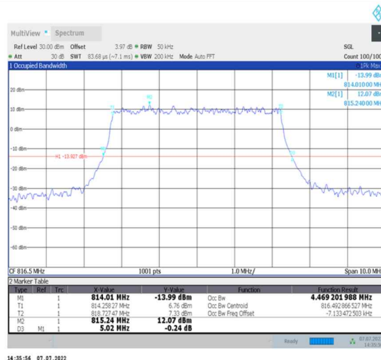
1-N26-814-824--15-5-L-4-DFT-64QAM-Outer_Full-25@0-Ant0-4.469-5.020-≤5-PASS
