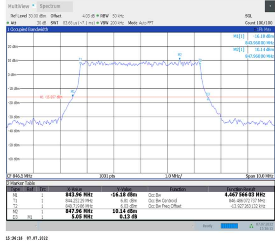
1-N26-824-849--15-5-H-8-CP-64QAM-Outer_Full-25@0-Ant0-4.468-5.050-≤5-PASS
