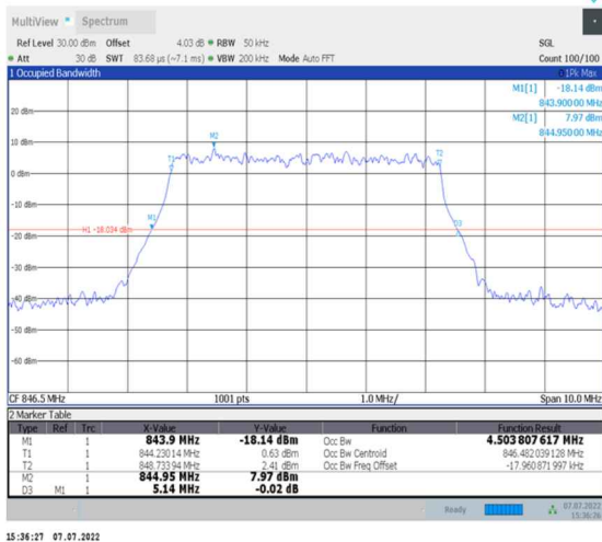
1-N26-824-849--15-5-H-9-CP-256QAM-Outer_Full-25@0-Ant0-4.504-5.140-≤5-PASS
