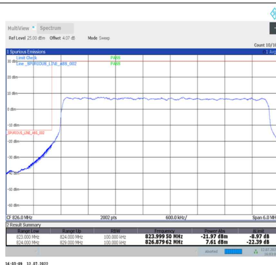
1-N26-824-849--15-5-L-3-DFT-PI2BPSK-Outer_Full-25@0-Ant0-seegraph-PASS-see graph
