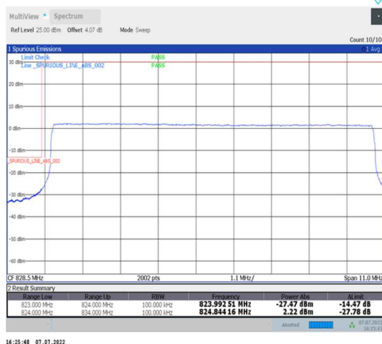
1-N26-824-849--15-10-L-6-CP-QPSK-Outer_Full-52@0-Ant0-seegraph-PASS-see graph
