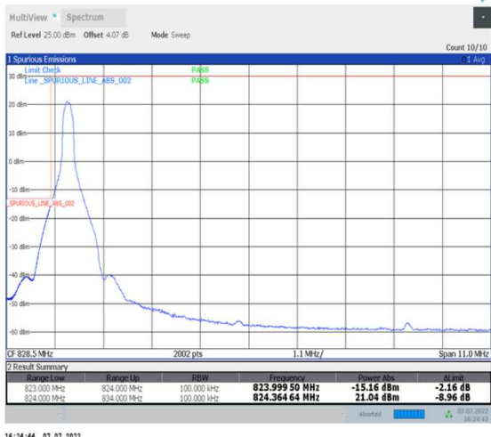
1-N26-824-849--15-10-L-1-DFT-PI2BPSK-Edge_1RB_Left-1@0-Ant0-seegraph-PASS-see graph
