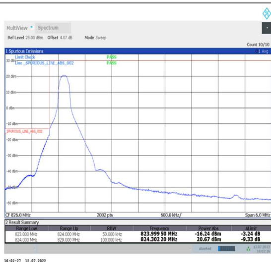
1-N26-824-849--15-5-L-1-DFT-PI2BPSK-Edge_1RB_Left-1@0-Ant0-seegraph-PASS-see graph
