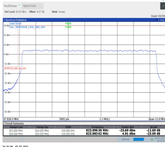
1-N26-824-849--15-10-L-3-DFT-PI2BPSK-Outer_Full-50@0-Ant0-seegraph-PASS-see graph
