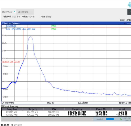
1-N26-824-849--15-5-L-4-CP-QPSK-Edge_1RB_Left-1@0-Ant0-seegraph-PASS-see graph
