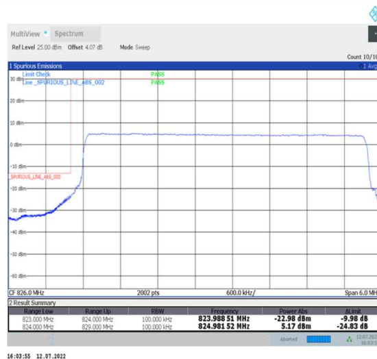
1-N26-824-849--15-5-L-6-CP-QPSK-Outer_Full-25@0-Ant0-seegraph-PASS-see graph
